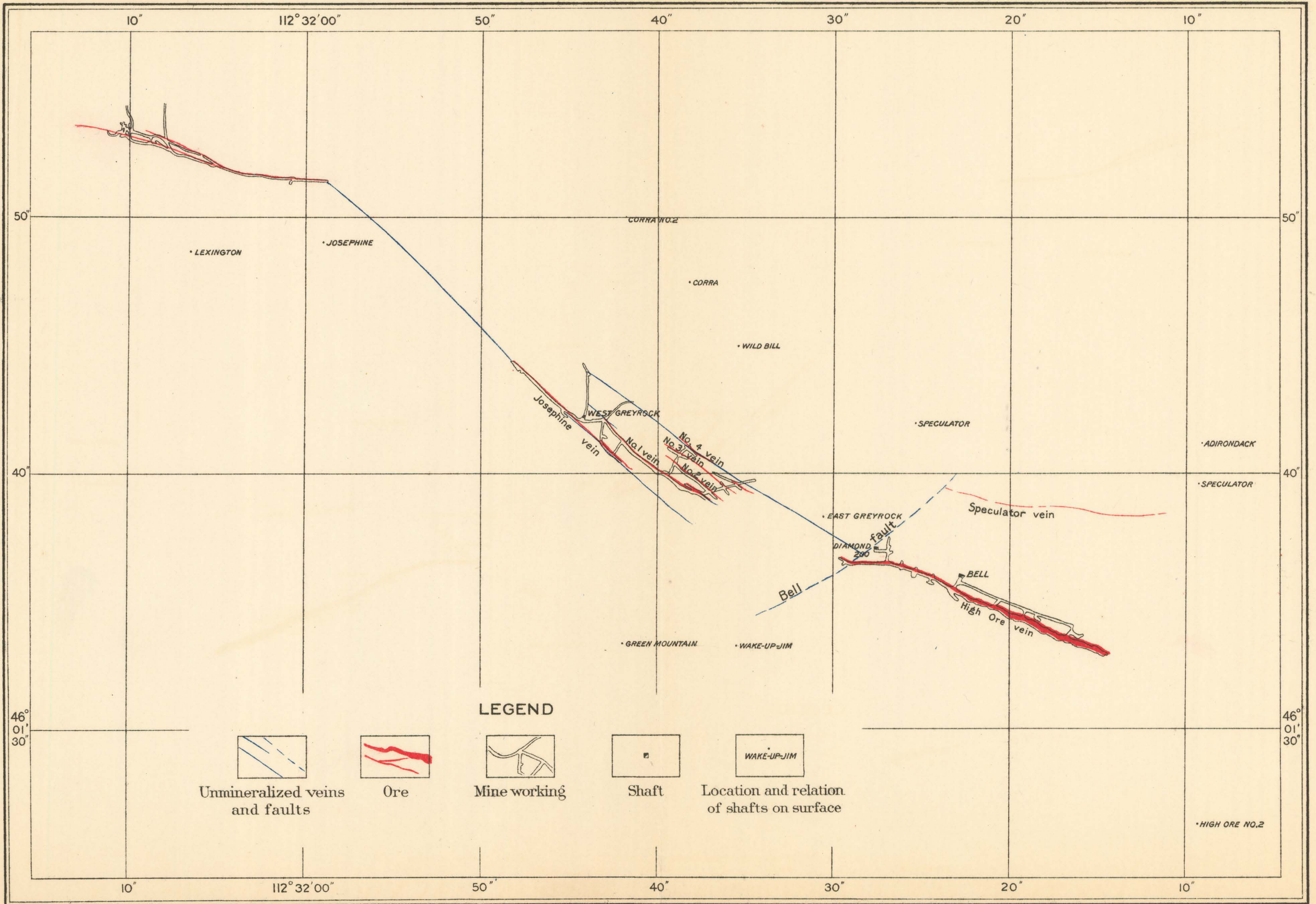
MAP SHOWING KNOWN VEIN STRUCTURE ON 6100-FOOT PLANE ABOVE SEA LEVEL
