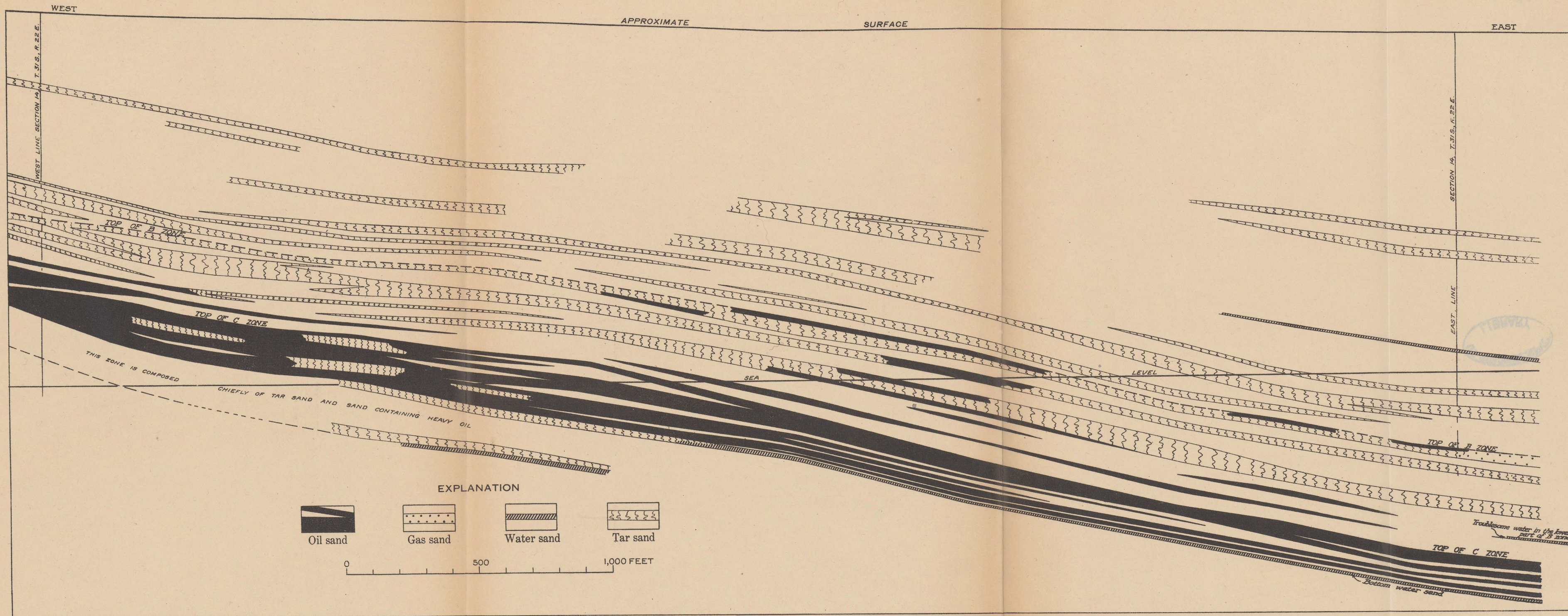
GEOLOGIC SECTION ALONG EAST-WEST CENTER LINE OF SEC. 14, T. 31 S., R. 22 E. (SEE LINE A-A', PLATE III)
