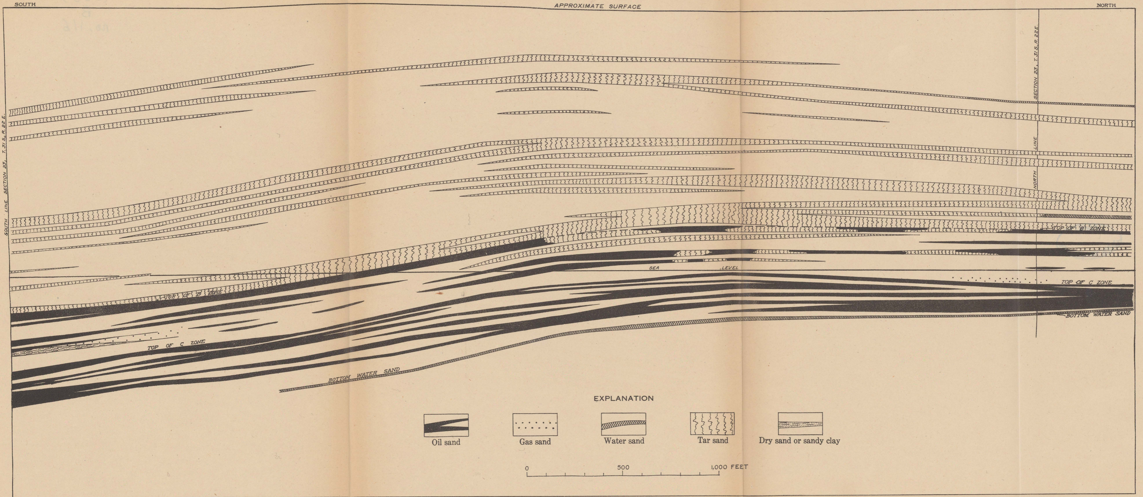
GEOLOGIC SECTION ALONG NORTH-SOUTH CENTER LINE OF SEC. 23, T. 31 S., R. 22 E. (SEE LINE 'B-B', PLATE III)
