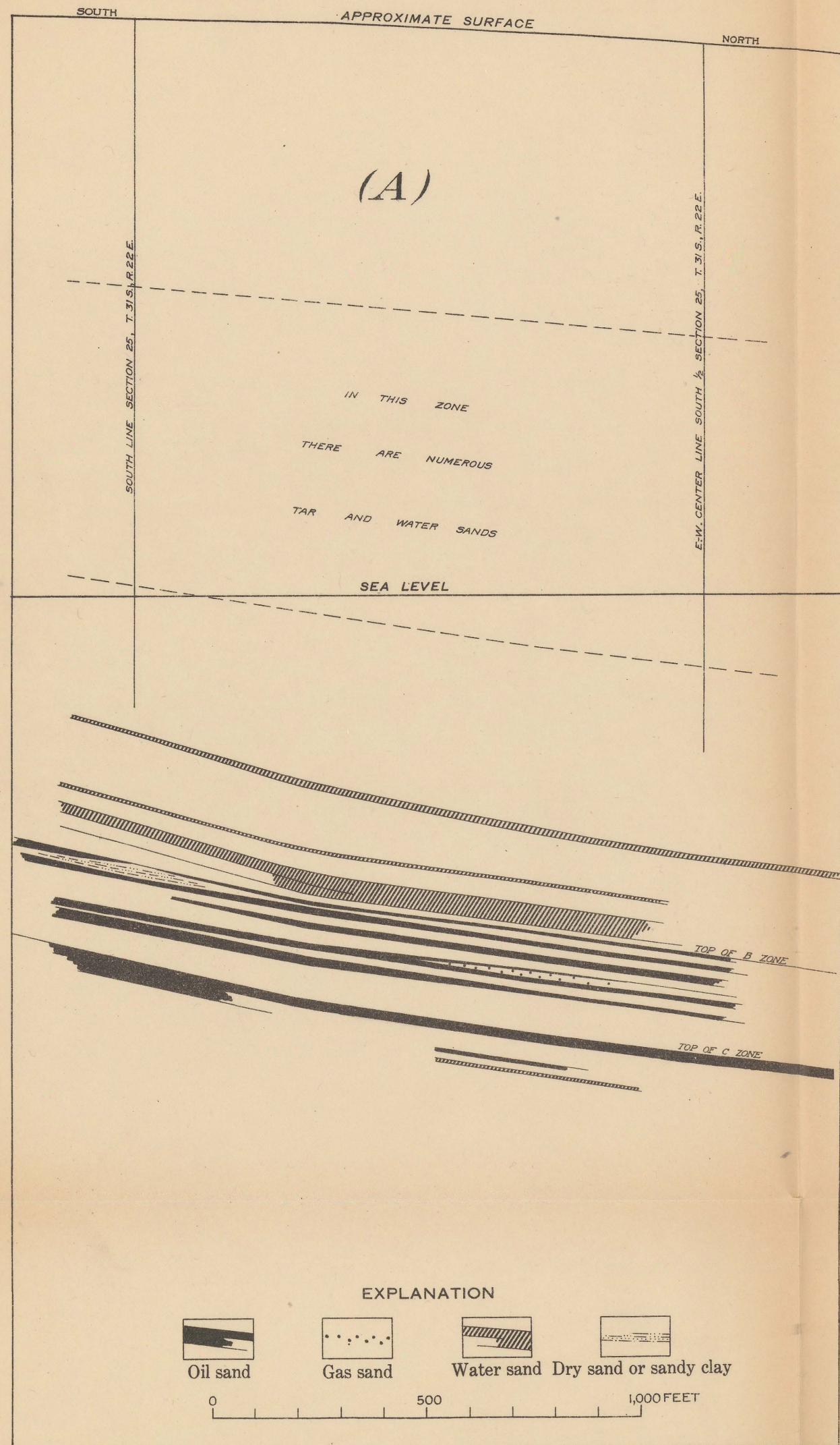
GEOLOGIC SECTION ALONG WEST LINE S.½ SE.¼ SEC. 25, T. 31 S., R. 22 E. (SEE LINE C-C', PLATE III)
