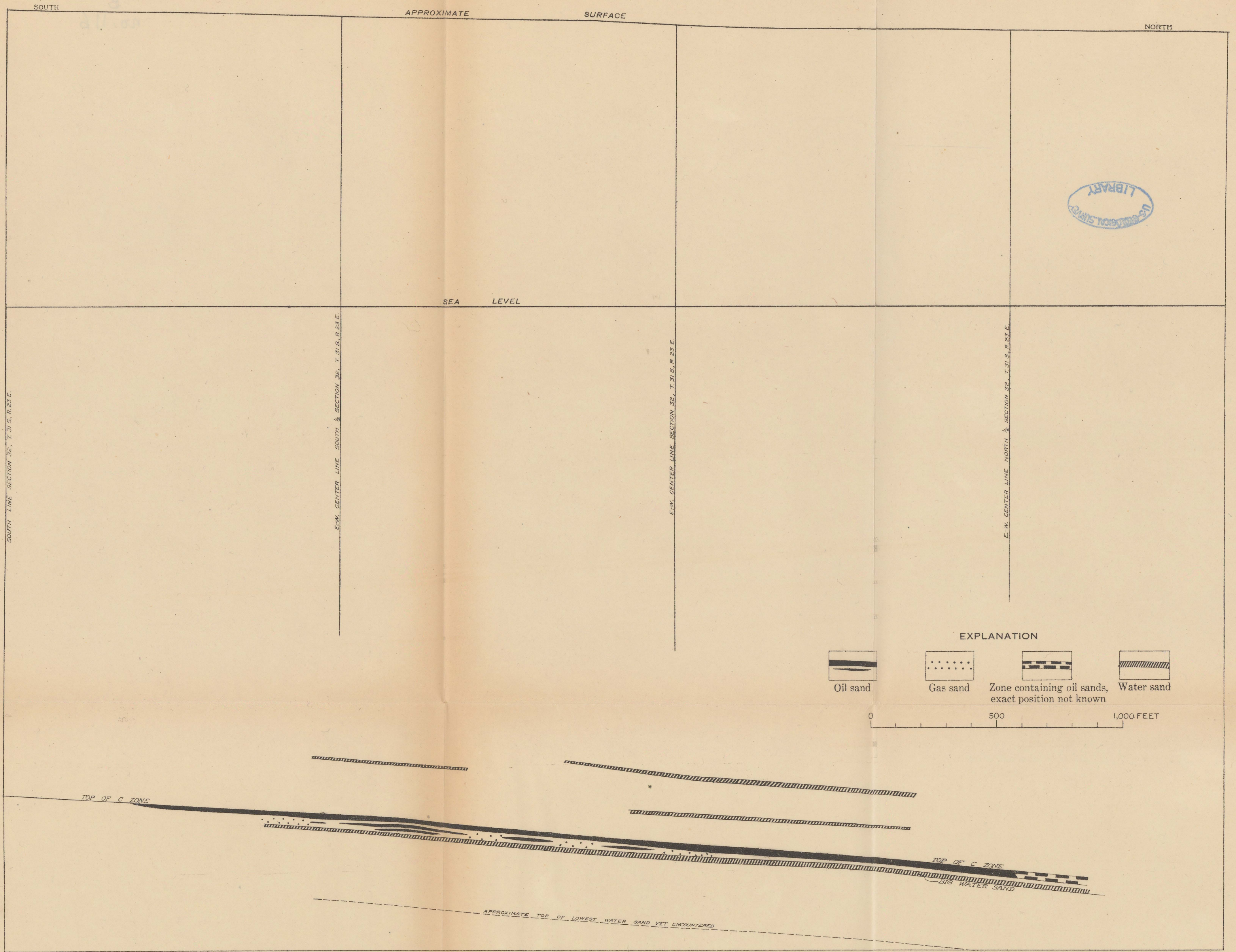
GEOLOGIC SECTION ALONG EAST LINE OF PACIFIC CRUDE PROPERTY, SE. 1/4 SEC. 32, T. 31 S., R. 23 E. (SEE LINE E-E', PLATE III)
