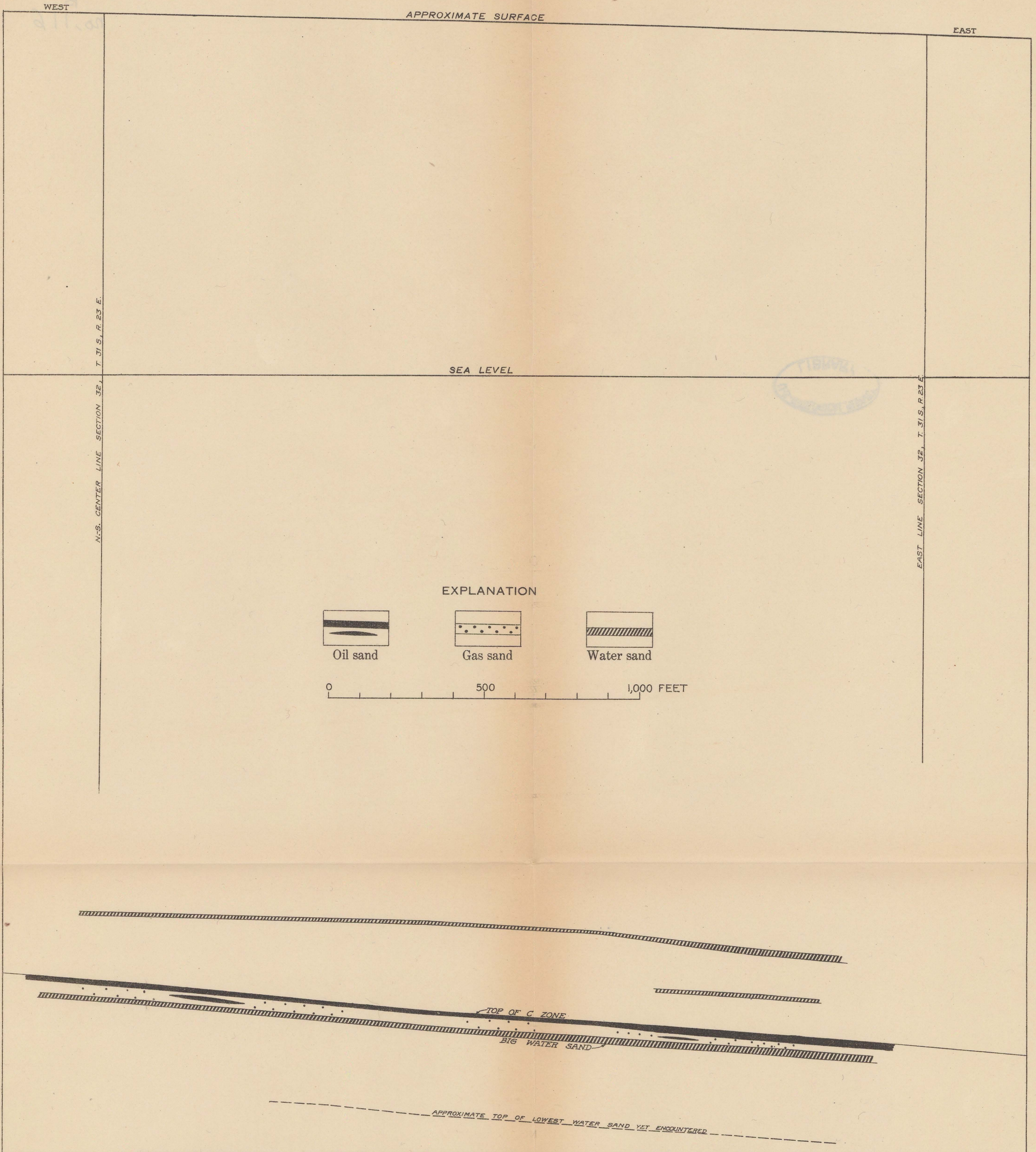
GEOLOGIC SECTION ALONG SOUTH LINE OF NE. 1/4 SEC. 32, T. 31 S., R. 23 E. (SEE LINE F-F', PLATE III)
