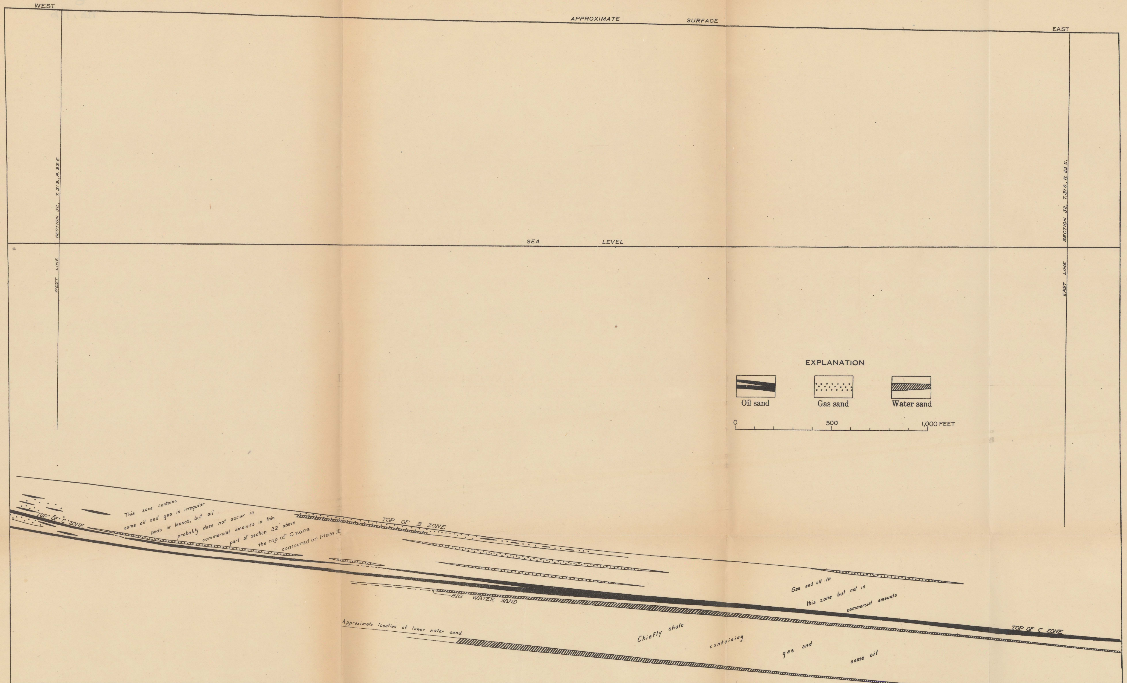
GEOLOGIC SECTION ALONG EAST-WEST CENTER LINE OF S. 1/2 SEC. 32, T. 31 S., R. 23 E. (SEE LINE G-G', PLATE III)
