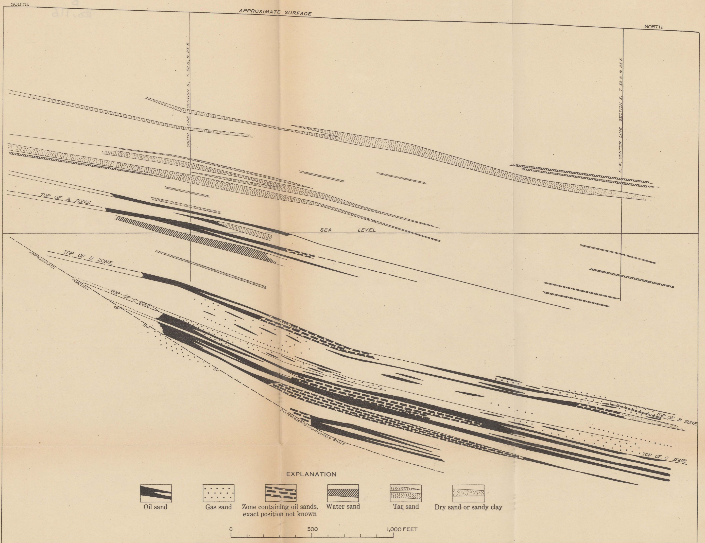
GEOLOGIC SECTION ALONG WEST LINE OF SE. 1/4 SEC. 5, T. 32 S., R. 23 E. (SEE LINE H-H', PLATE III)
