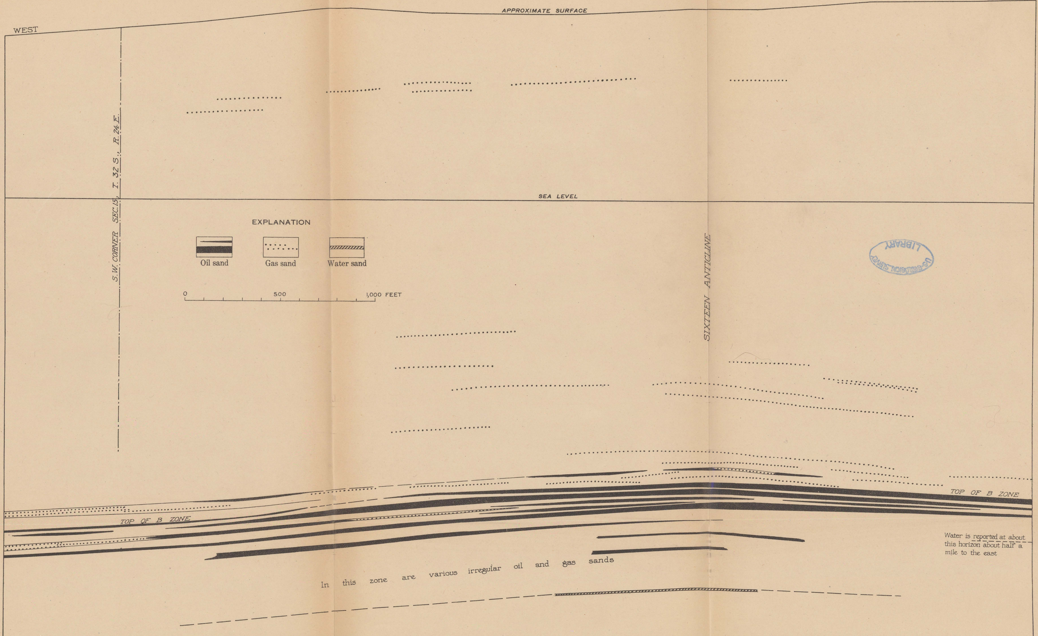
GEOLOGIC SECTION ALONG NORTH LINE OF SEC. 16, T. 32 S., R. 24 E. (SEE LINE L-L', PLATE III)
