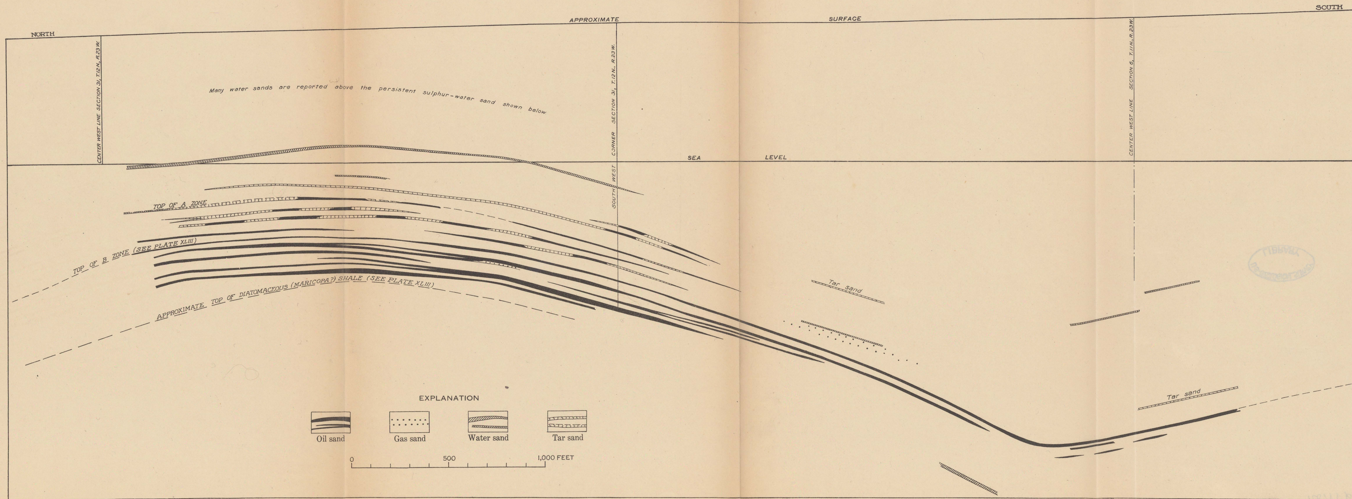
GEOLOGIC SECTION ALONG WEST LINE OF NW.¼ SEC. 6, T. 11 N., R. 23 W., AND SW.¼ SEC. 31, T. 12 N., R. 23 W. (SEE LINE M-M', PLATE III)
