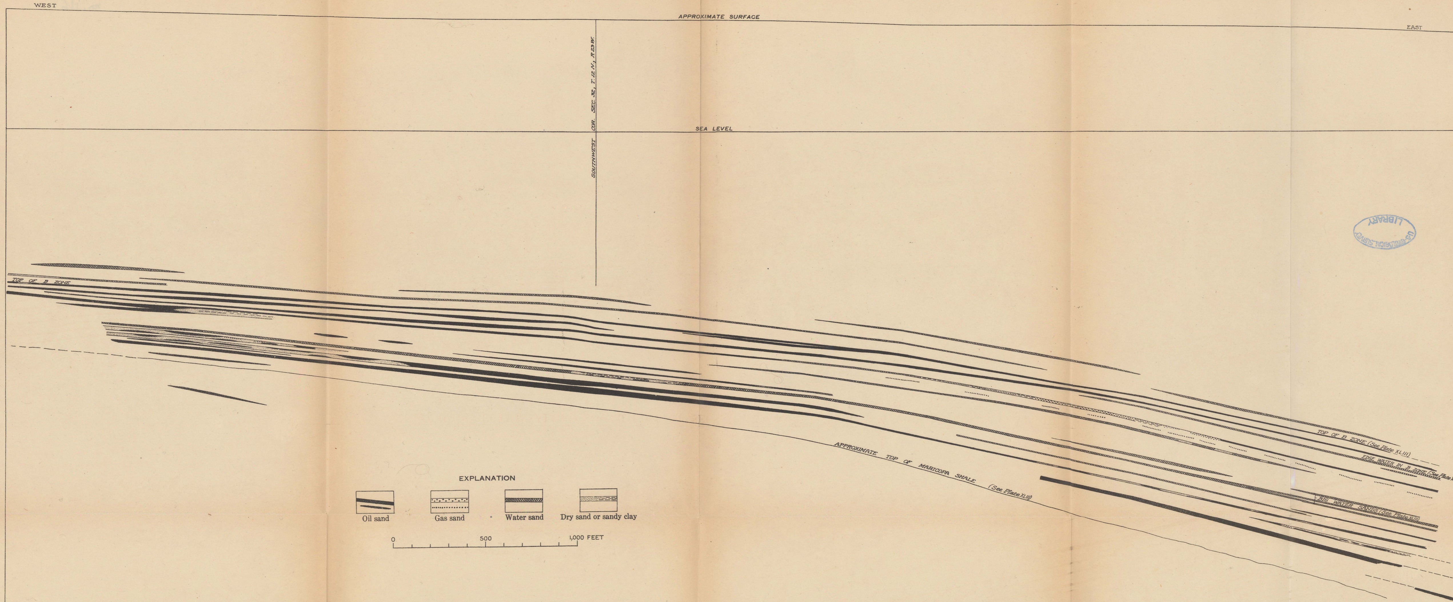
GEOLOGIC SECTION ALONG SOUTH LINE OF SECS. 31 AND 32, T. 12 N., R. 23 W. (SEE LINE N-N', PLATE III)
