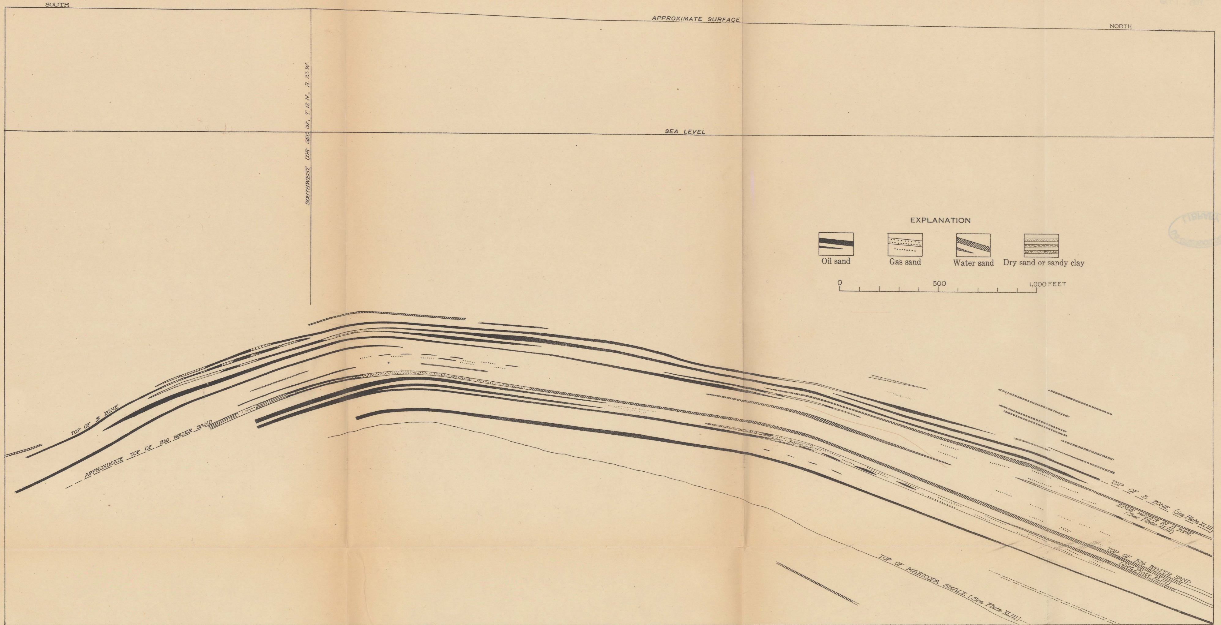
GEOLOGIC SECTION ALONG WEST LINE OF SEC. 32, T. 12 N., R. 23 W. (SEE LINE P-P', PLATE III)
