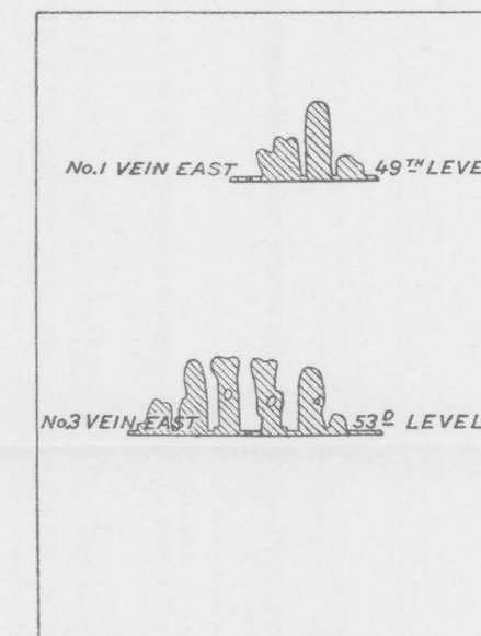
STOPE PLAN OF No. 1 VEIN EAST 49 th LEVEL AND No. 3 VEIN EAST 53 d LEVEL
