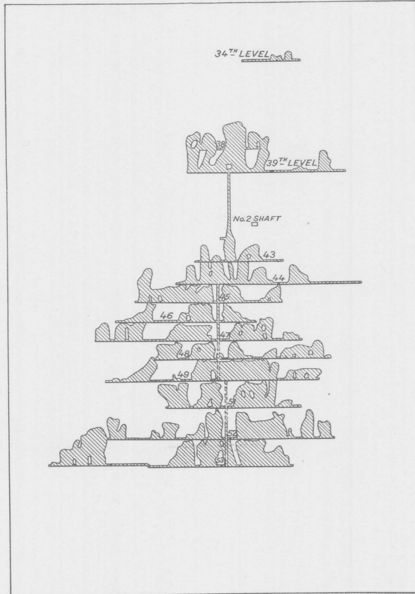
STOPE PLAN OF No. 4 VEIN
