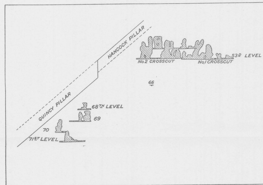
STOPE PLAN OF HANGING VEIN
