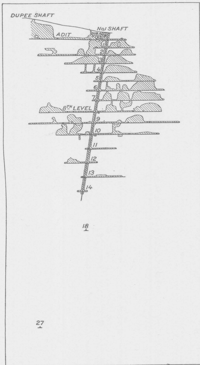
STOPE PLAN OF No. 1 VEIN
