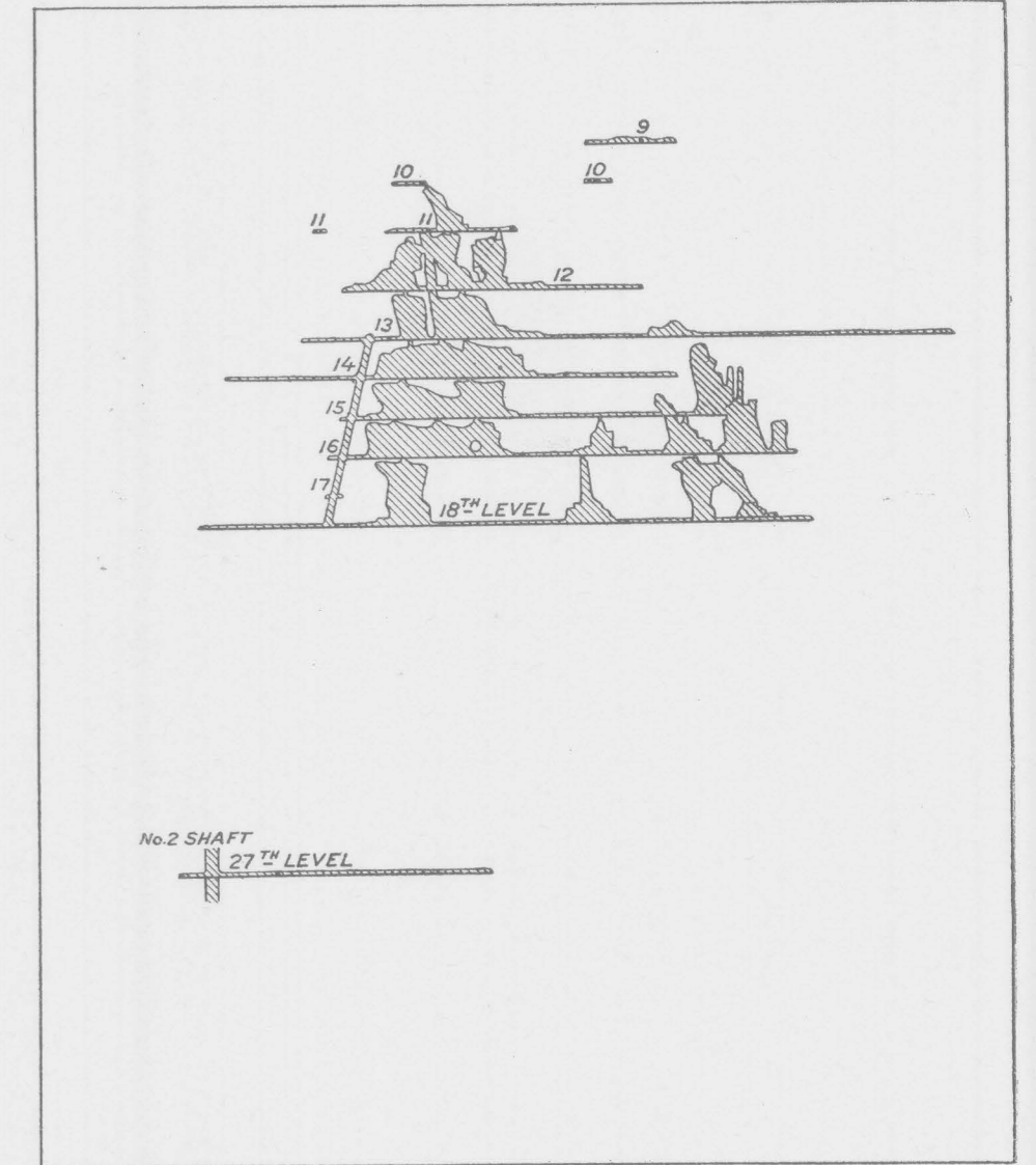
STOPE PLAN OF No. 3 VEIN
