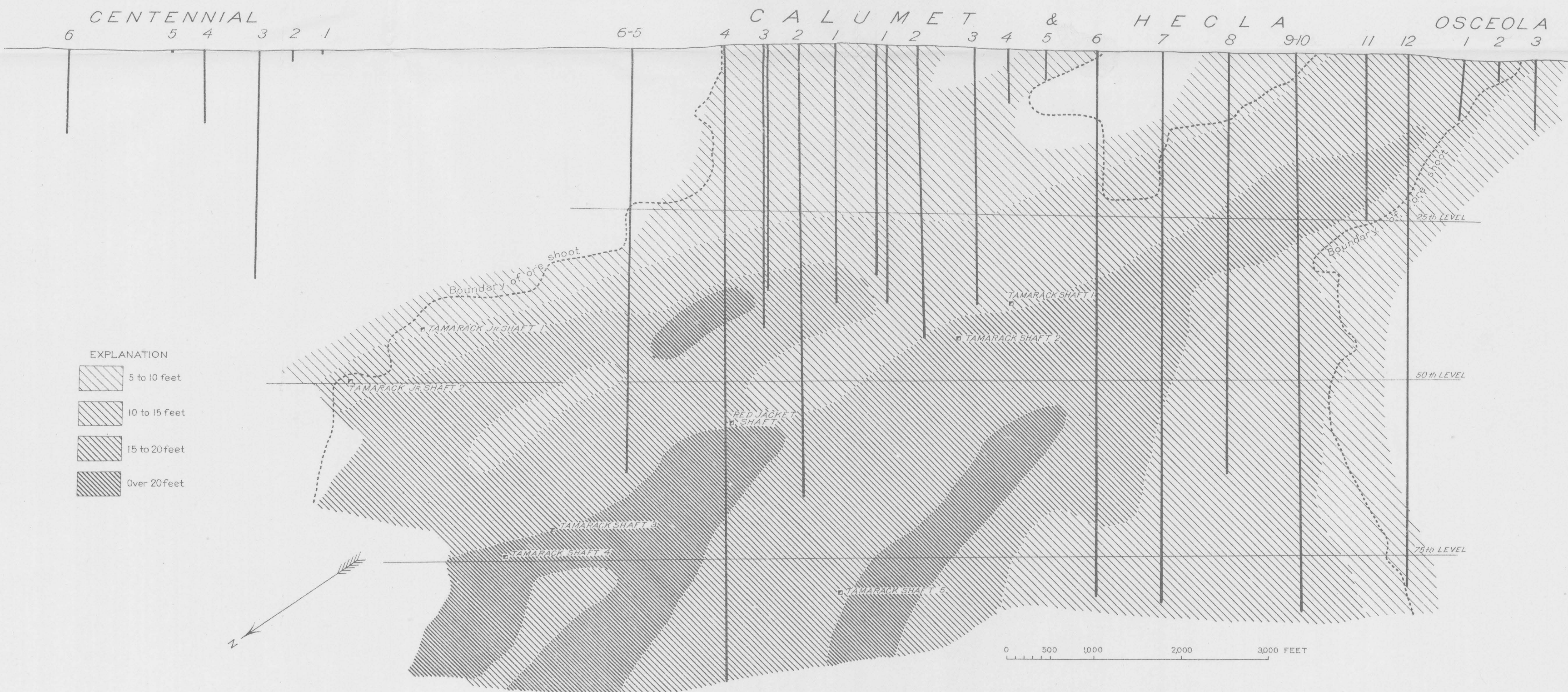
PLAN SHOWING THICKNESS OF LODGE
