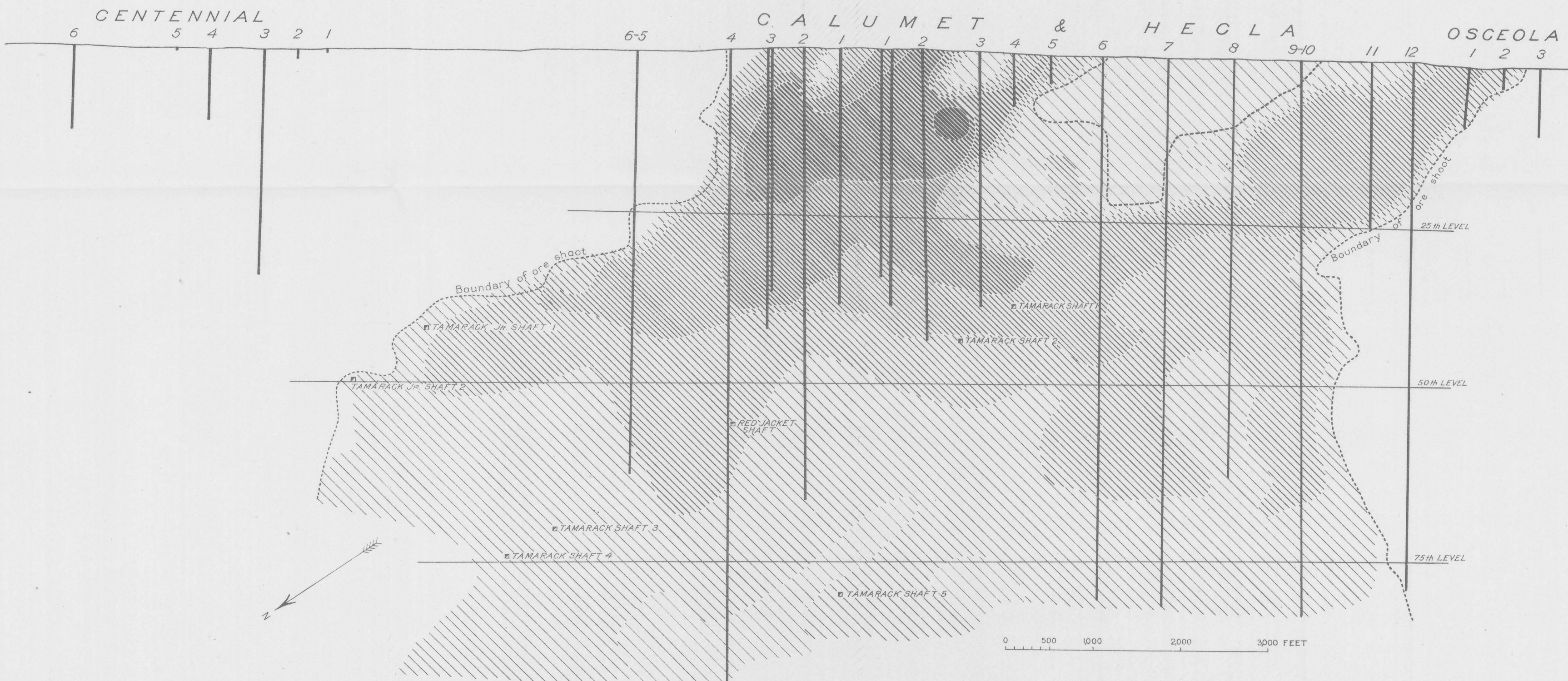
PLAN SHOWING RELATIVE COPPER CONTENT PER TON Darker shading indicates higher grades PLANS OF CALUMET AND HECLA CONGLOMERATE MINE
