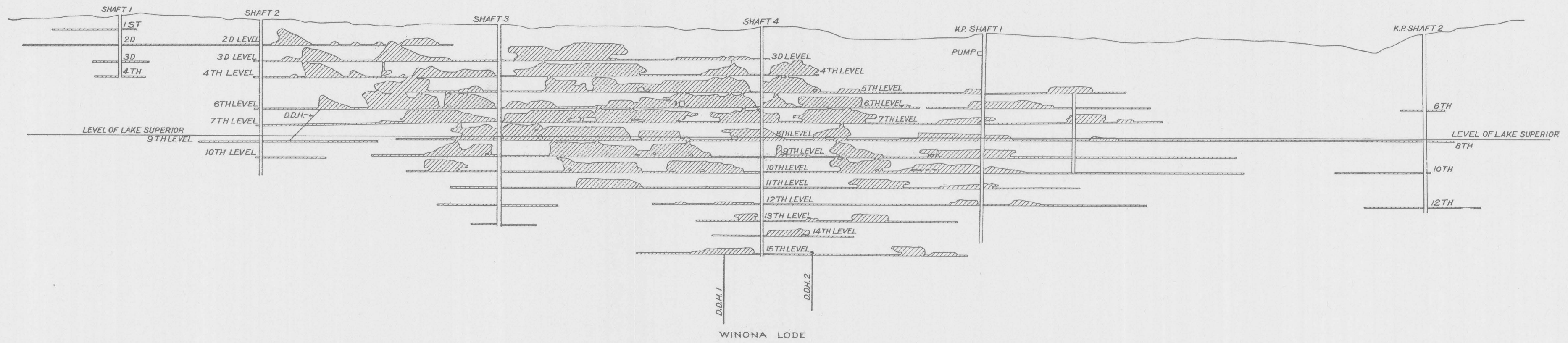
LONGITUDINAL SECTIONS OF OLD ARCADIAN AND WINONA LODES
