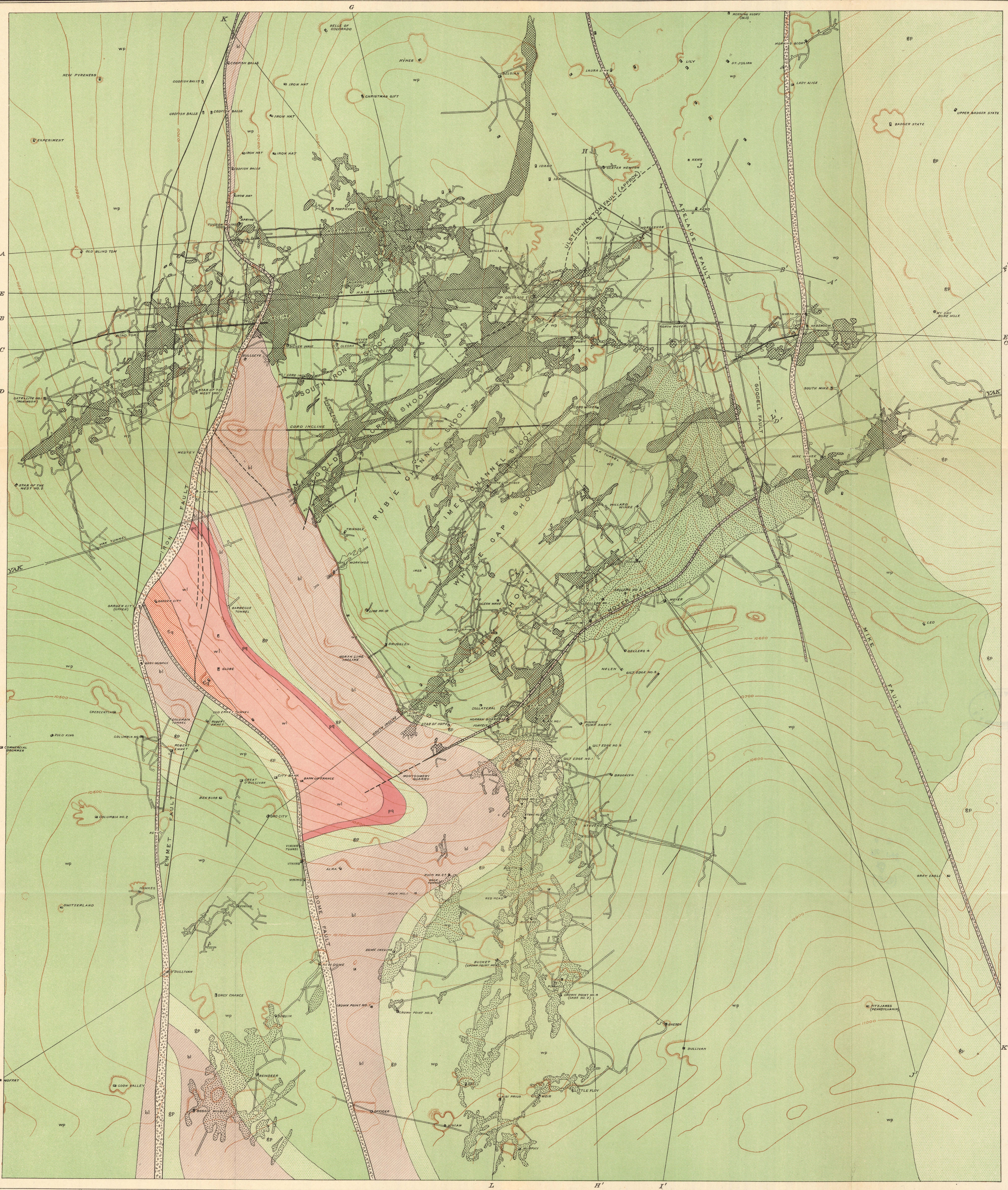
GEOLOGIC MAP OF IRON AND DOME HILLS, LEADVILLE MINING DISTRICT, COLORADO
