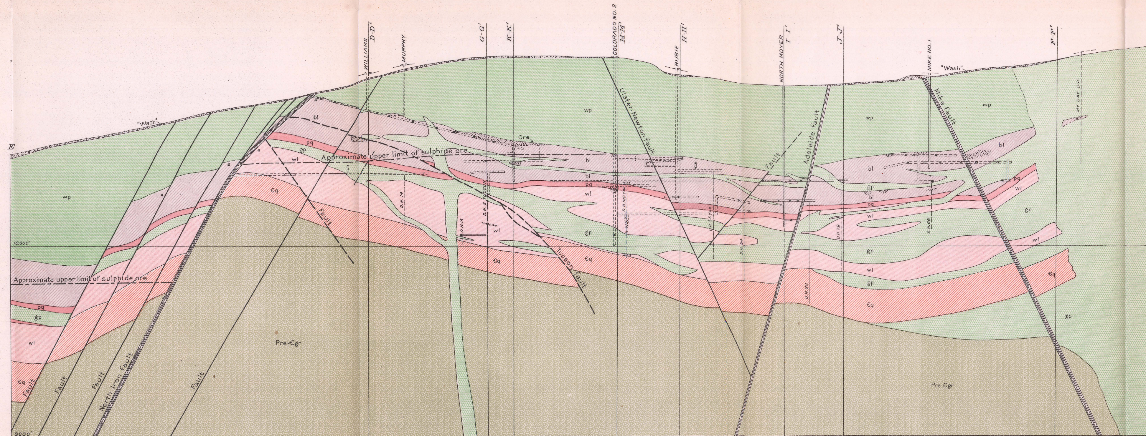
Section E-E'
