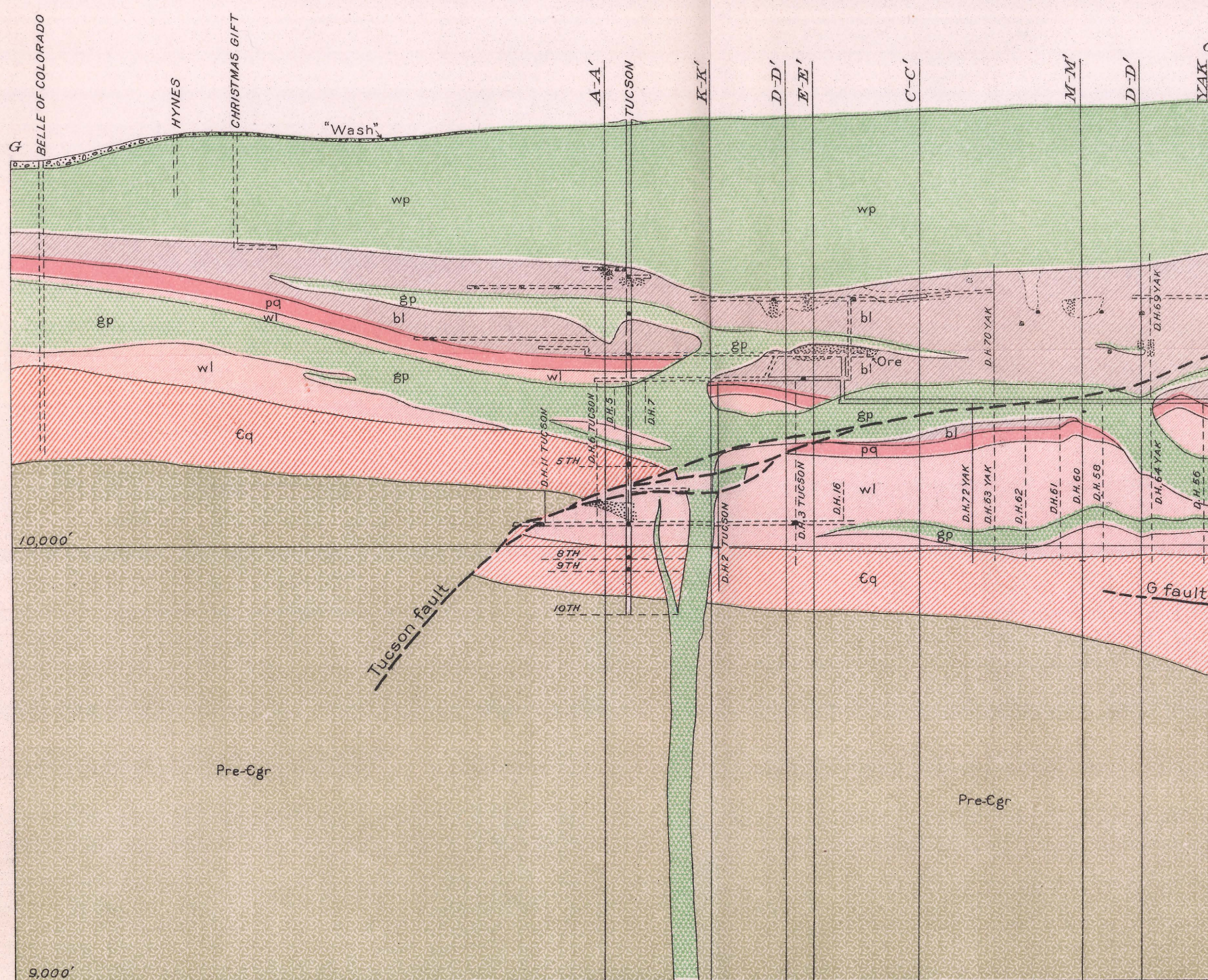
Section G-G'
