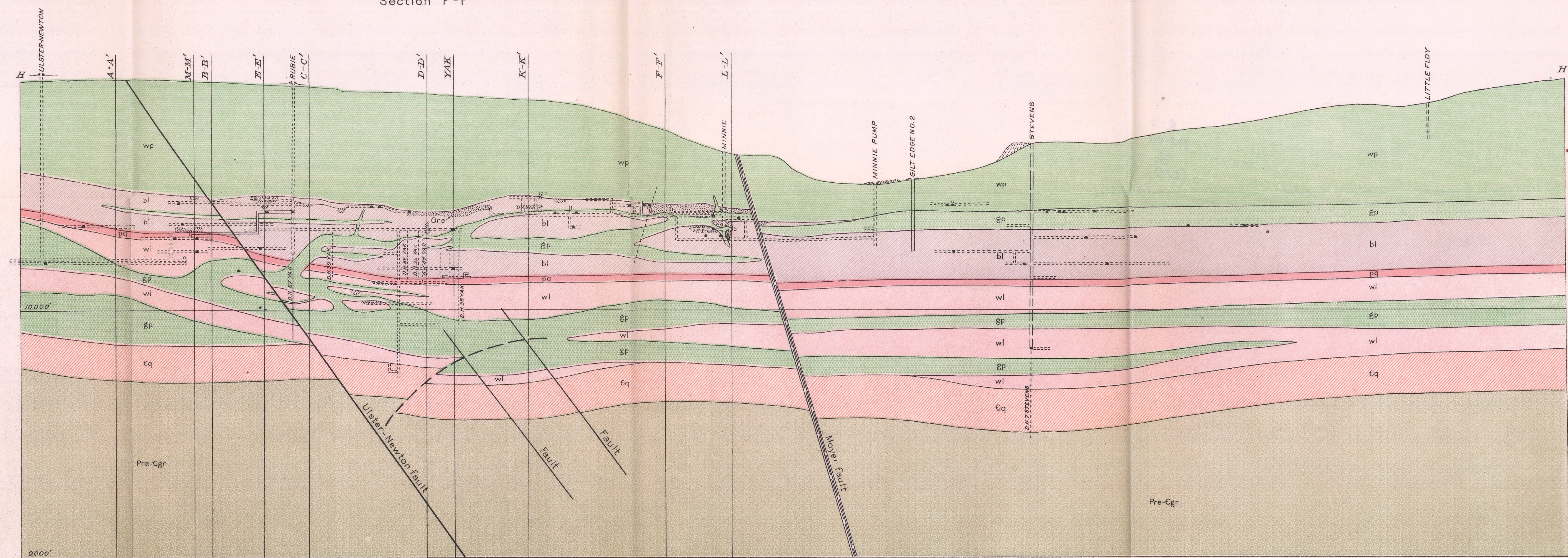
Section H-H'
