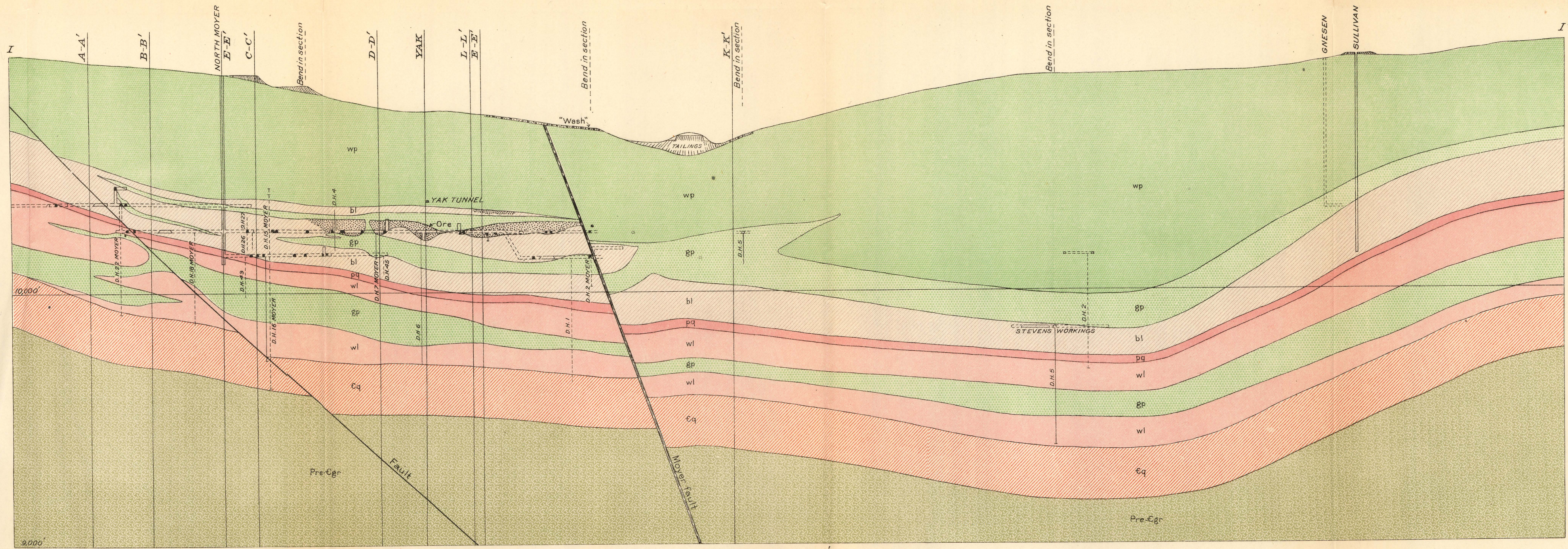
Section I-I'
