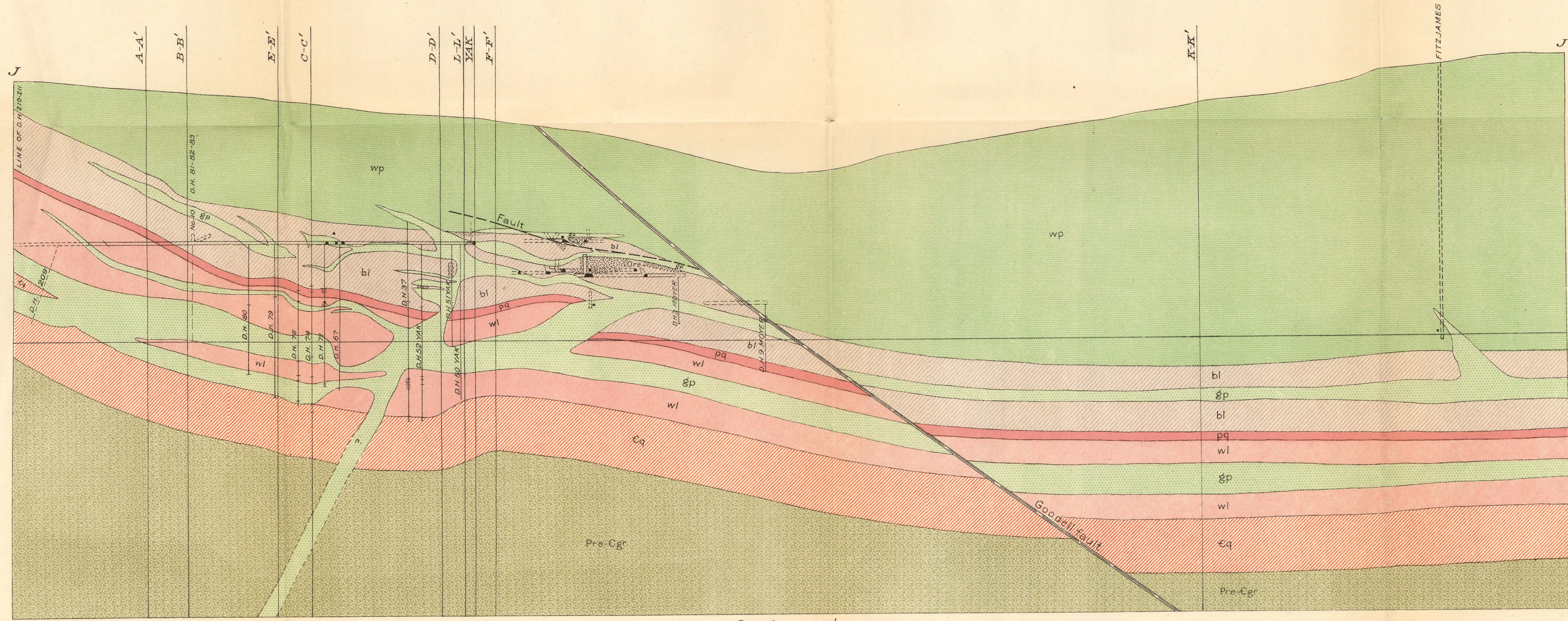
Section J-J'
