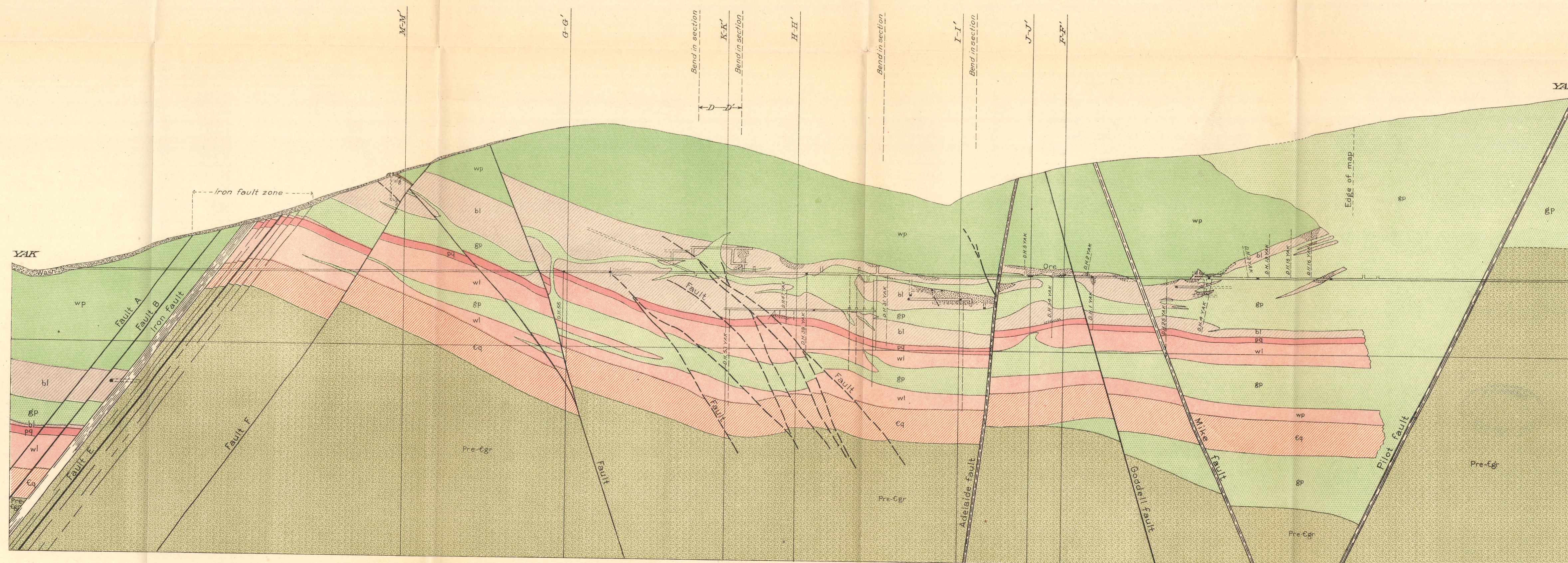
GEOLOGIC SECTIONS ALONG LINES L-L' TO YAK, PLATE 22, IRON AND DOME HILLS, LEADVILLE MINING DISTRICT, COLORADO
