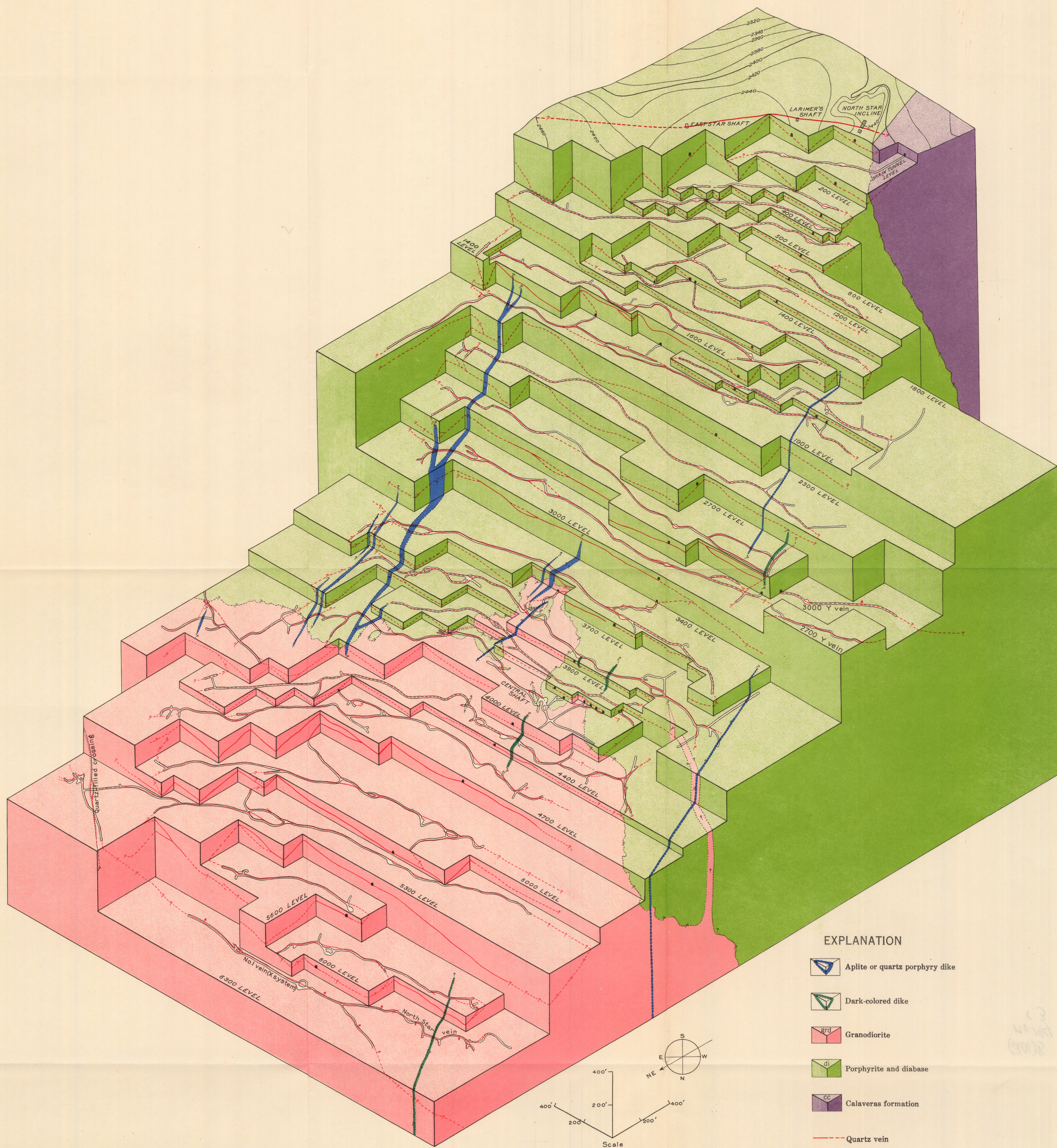
ISOMETRIC BLOCK DIAGRAM OF THE NORTH STAR VEIN OF THE NORTH STAR MINE IN 1931
