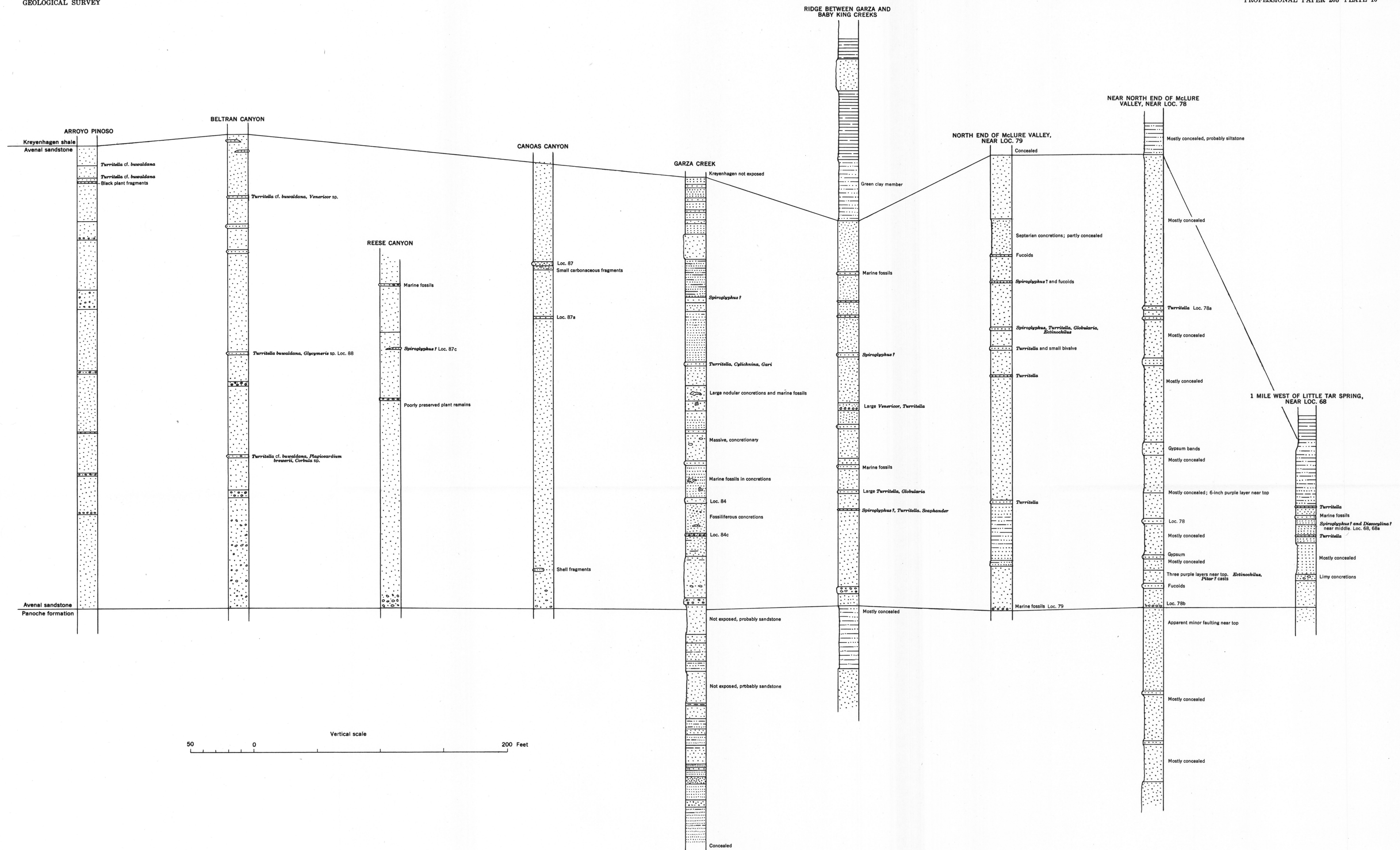
SECTIONS OF AVENAL SANDSTONE IN REEF RIDGE AREA
