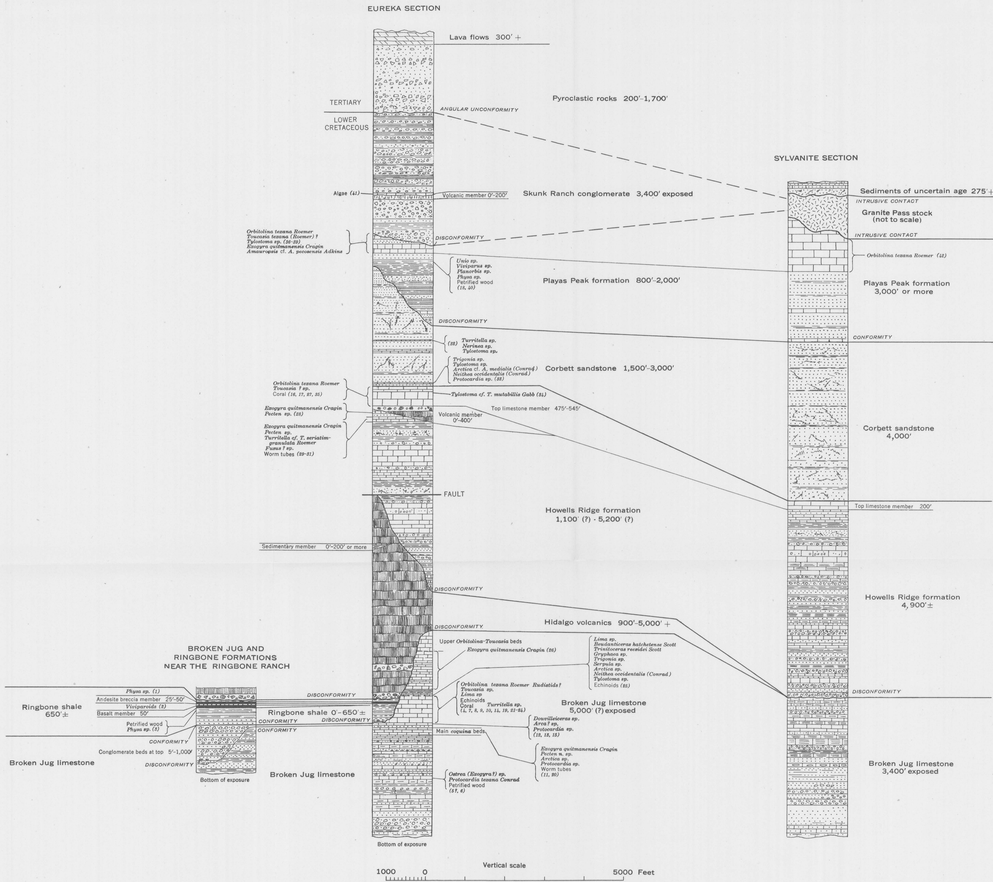
COMPARATIVE STRATIGRAPHIC COLUMNS SHOWING DISTRIBUTION OF FOSSIL ZONES Numbers following fossils refer to localities on plate 2
