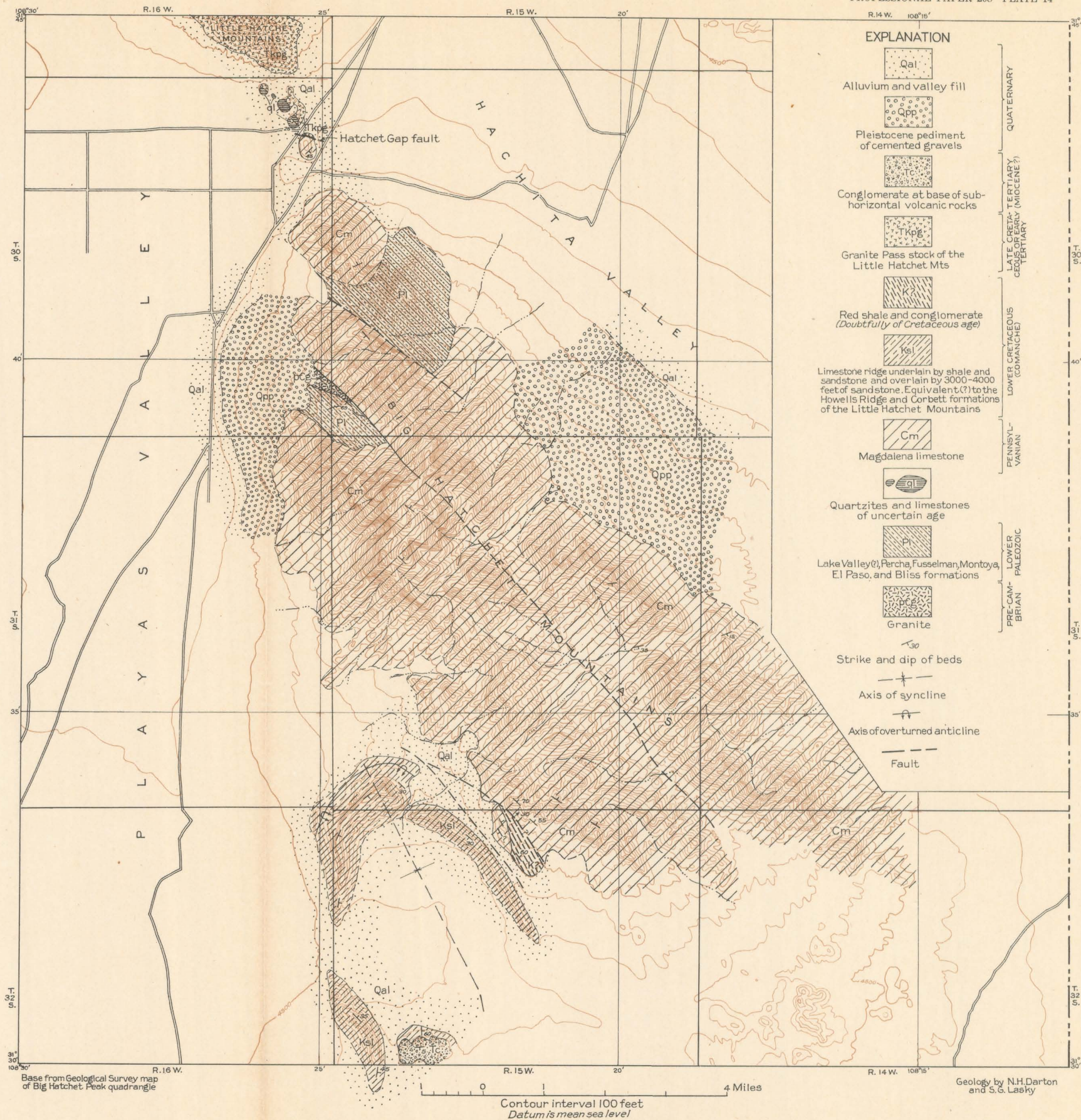
RECONNAISSANCE GEOLOGIC MAP OF THE BIG HATCHET MOUNTAINS, N. MEX.
