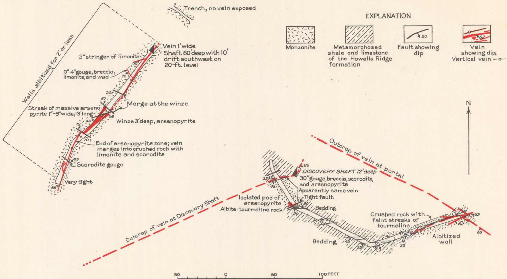
GEOLOGIC SKETCH MAP OF THE CREEPER TUNNELS
