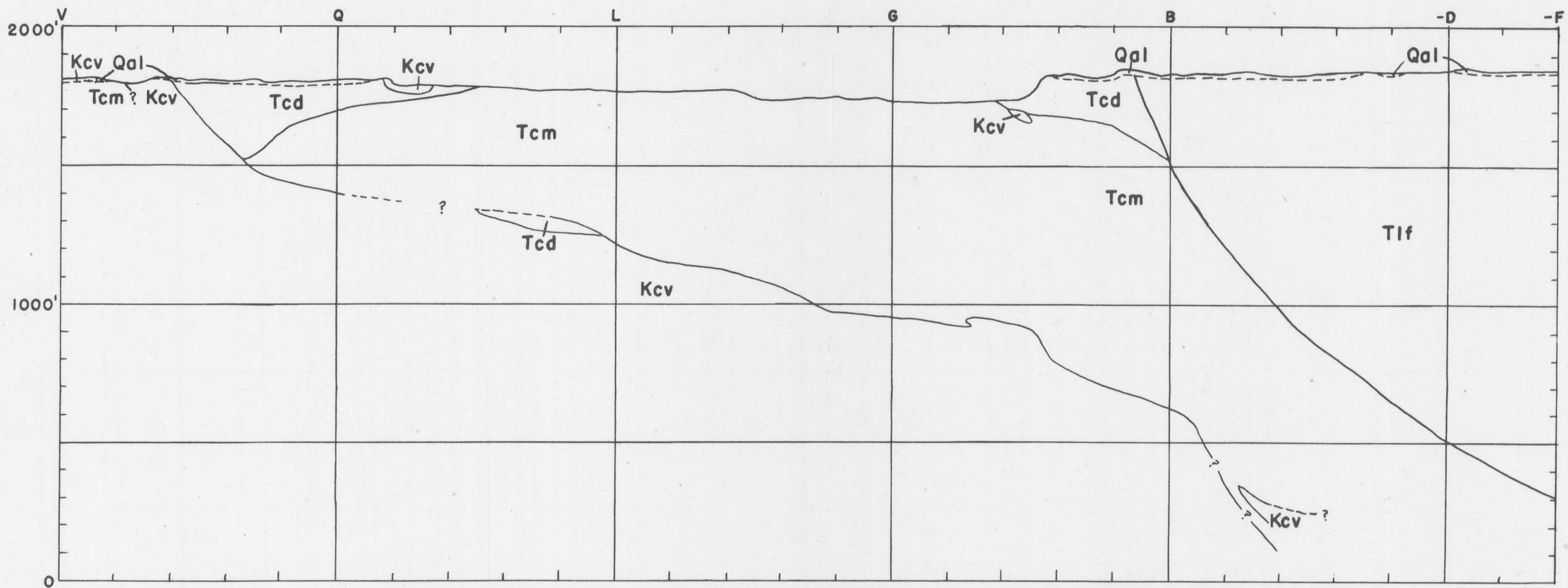
REVISED SECTION THROUGH COORDINATE 14
