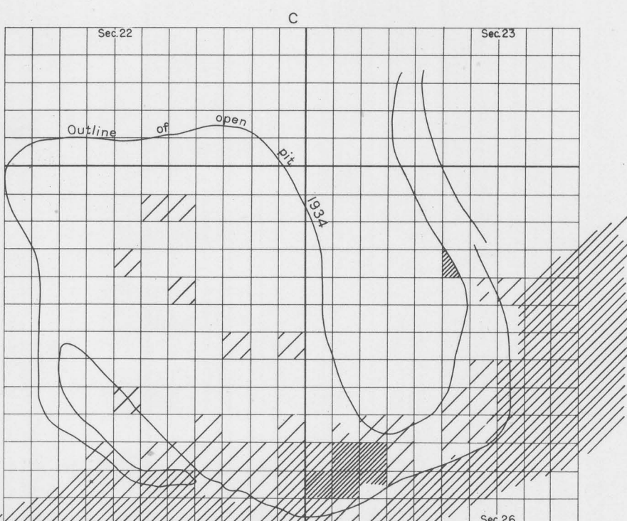
SPECULARITE
