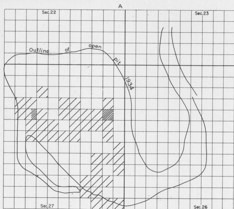
MOLYBDENITE
