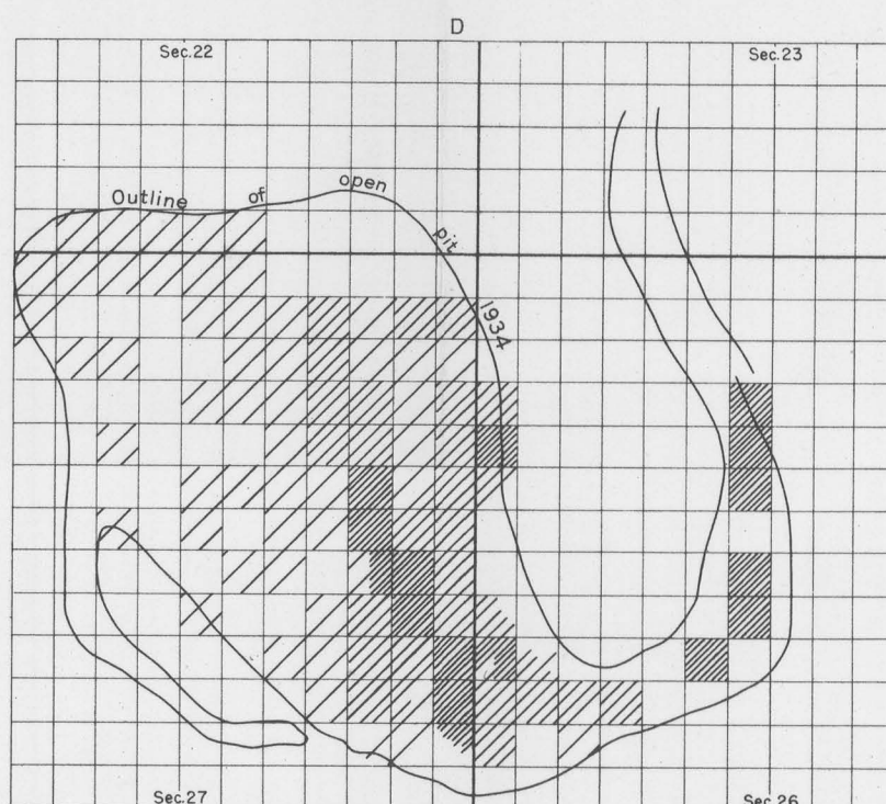
ESTIMATED PROPORTION OF PYRITE TO TOTAL SULFIDES
