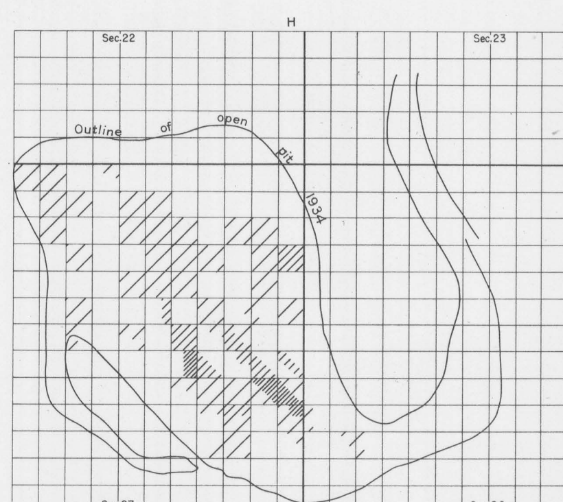
COARSE LEAFY CHLORITE AND BIOTITE
