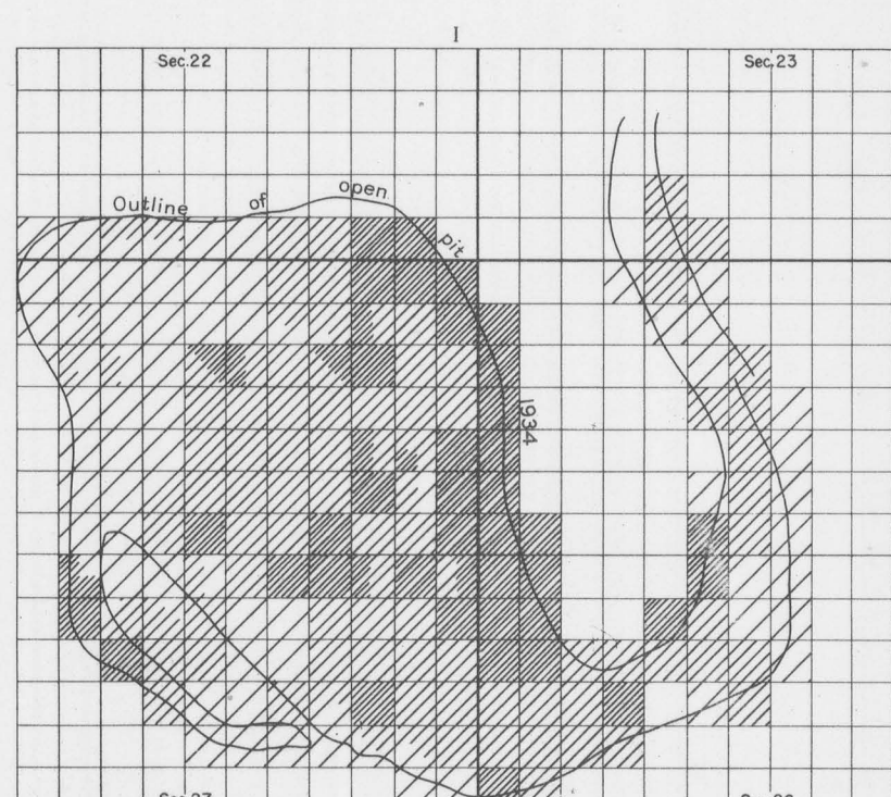
SERICITIZED PLAGIOCLASE
