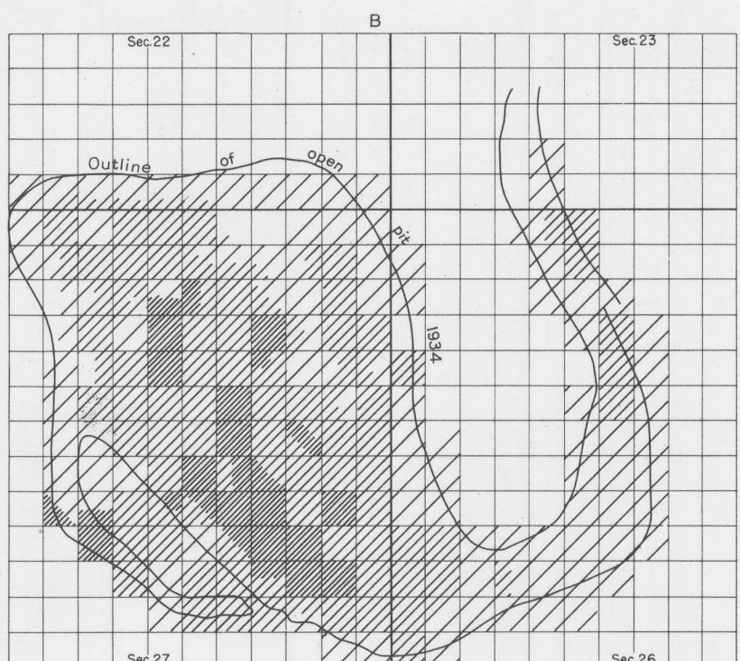
INTRODUCED QUARTZ
