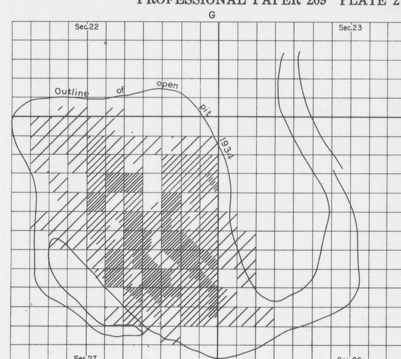
"INTRODUCED" ORTHOCLASE
