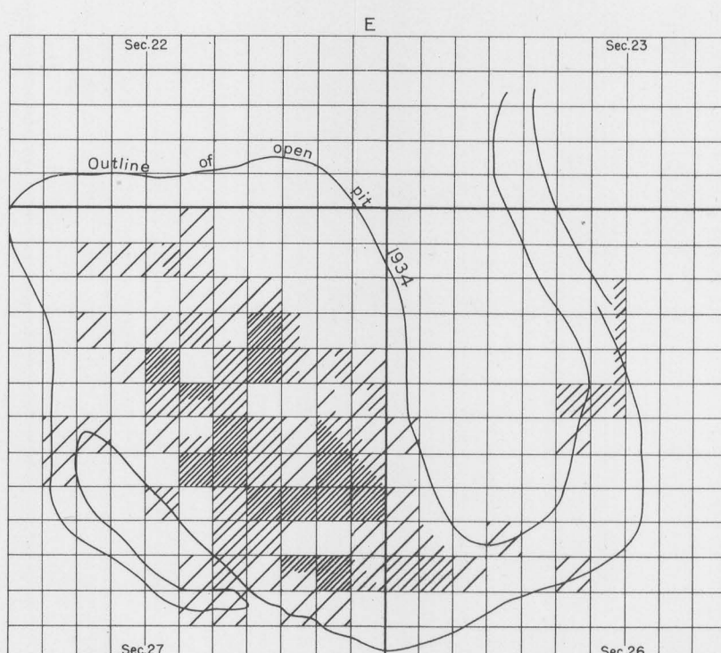
VEIN MAGNETITE
