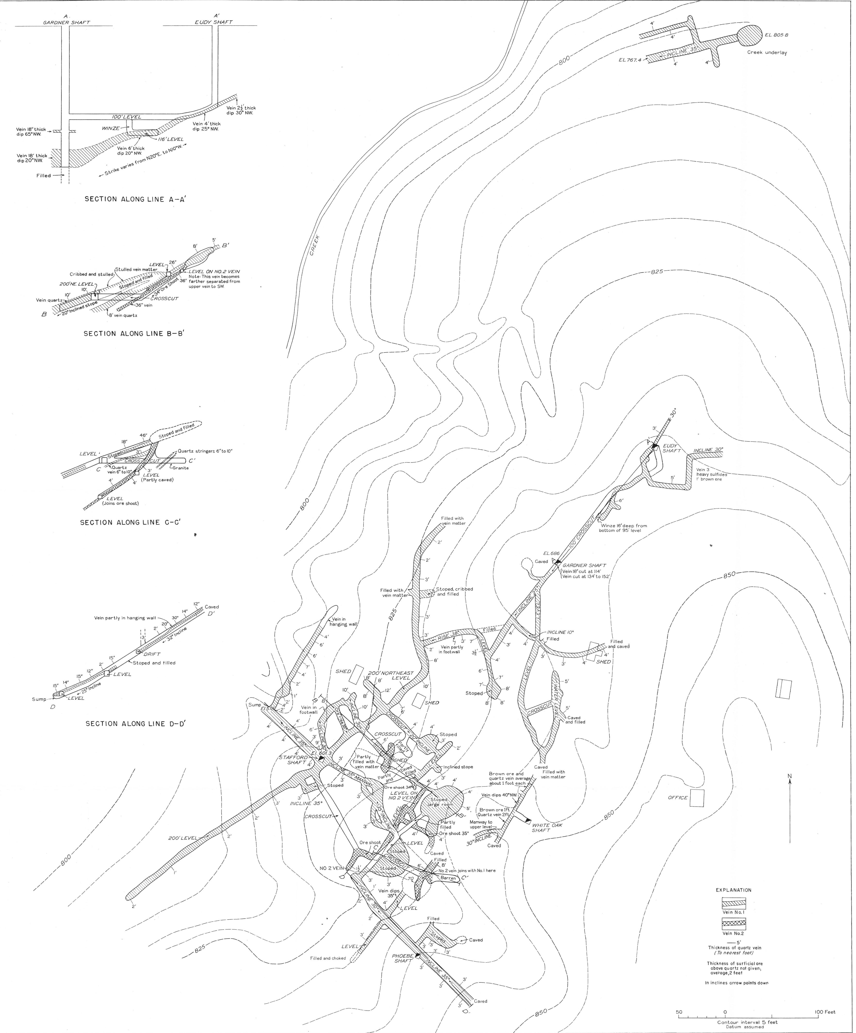
PLAN AND SECTIONS OF GARDNER HILL MINE, GUILFORD COUNTY, NORTH CAROLINA
