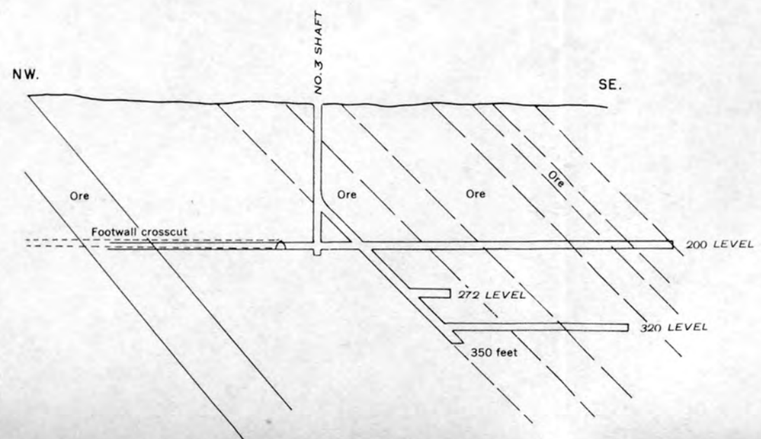
SECTION ON PLANE OF LODE THROUGH WORKINGS FROM NO. 3 SHAFT
