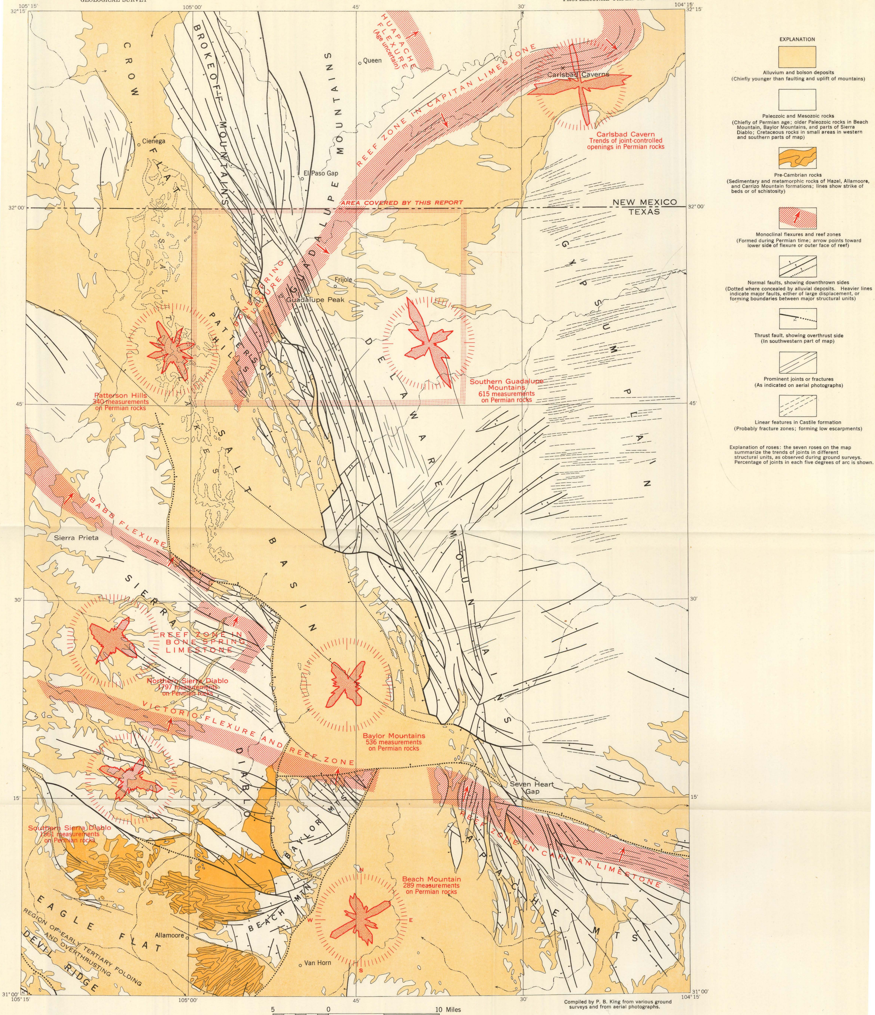
MAP OF GUADALUPE MOUNTAINS, TEXAS, AND SURROUNDING AREAS, SHOWING TECTONIC FEATURES
