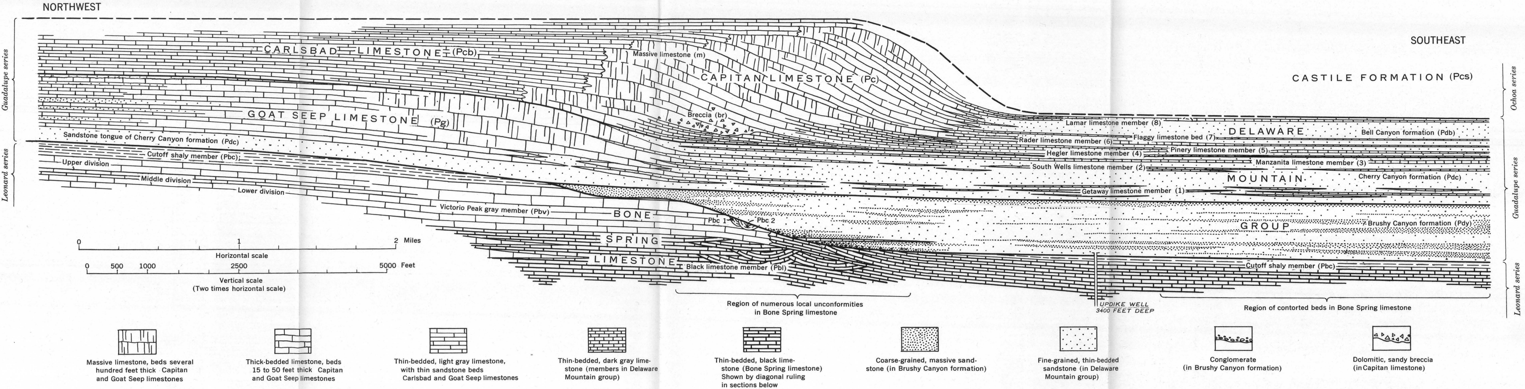
A. STRATIGRAPHIC DIAGRAM OF EXPOSED PERMIAN ROCKS
