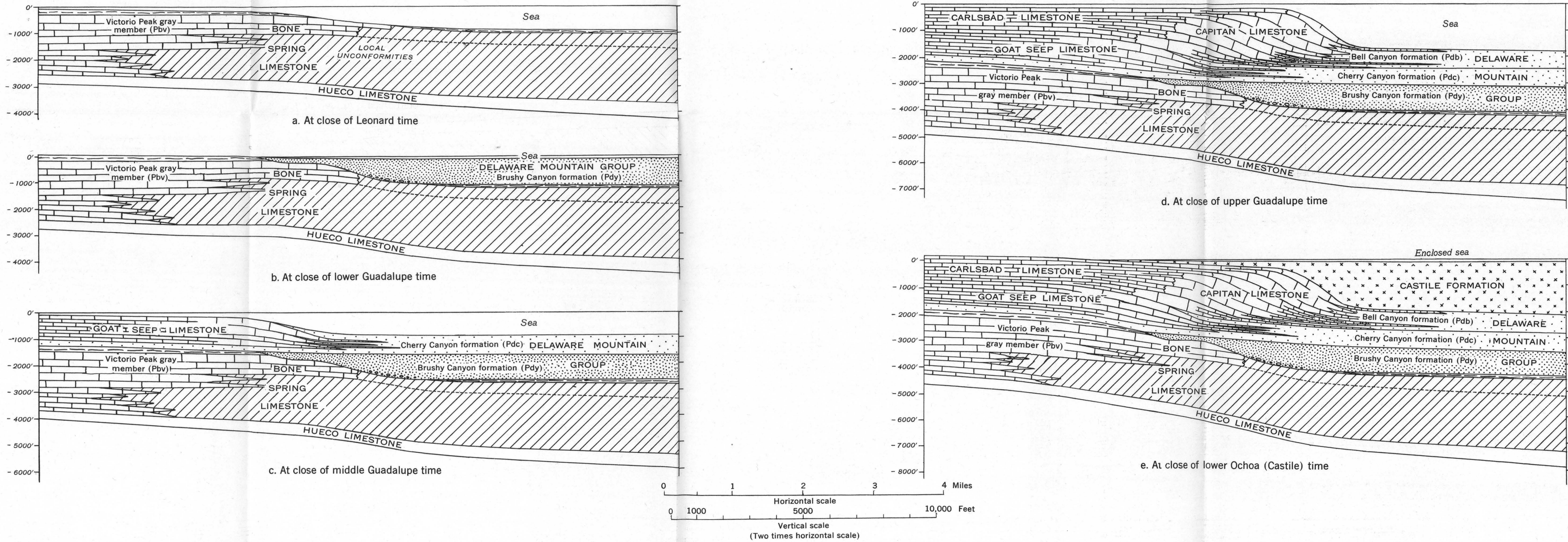
B. SECTIONS SHOWING STRUCTURE OF PERMIAN ROCKS AT SUCCESSIVE STAGES
