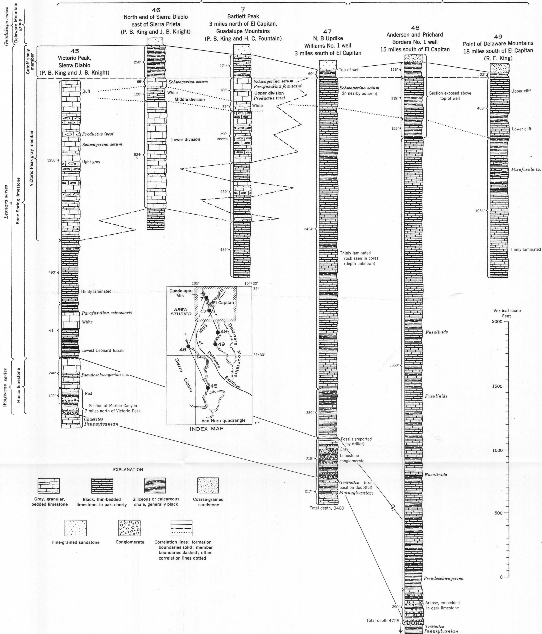
STRATIGRAPHIC SECTIONS OF BONE SPRING LIMESTONE IN SIERRA DIABLO, GUADALUPE, AND DELAWARE MOUNTAINS, TO ILLUSTRATE CORRELATION OF MEMBERS AND CHANGES IN THICKNESS
