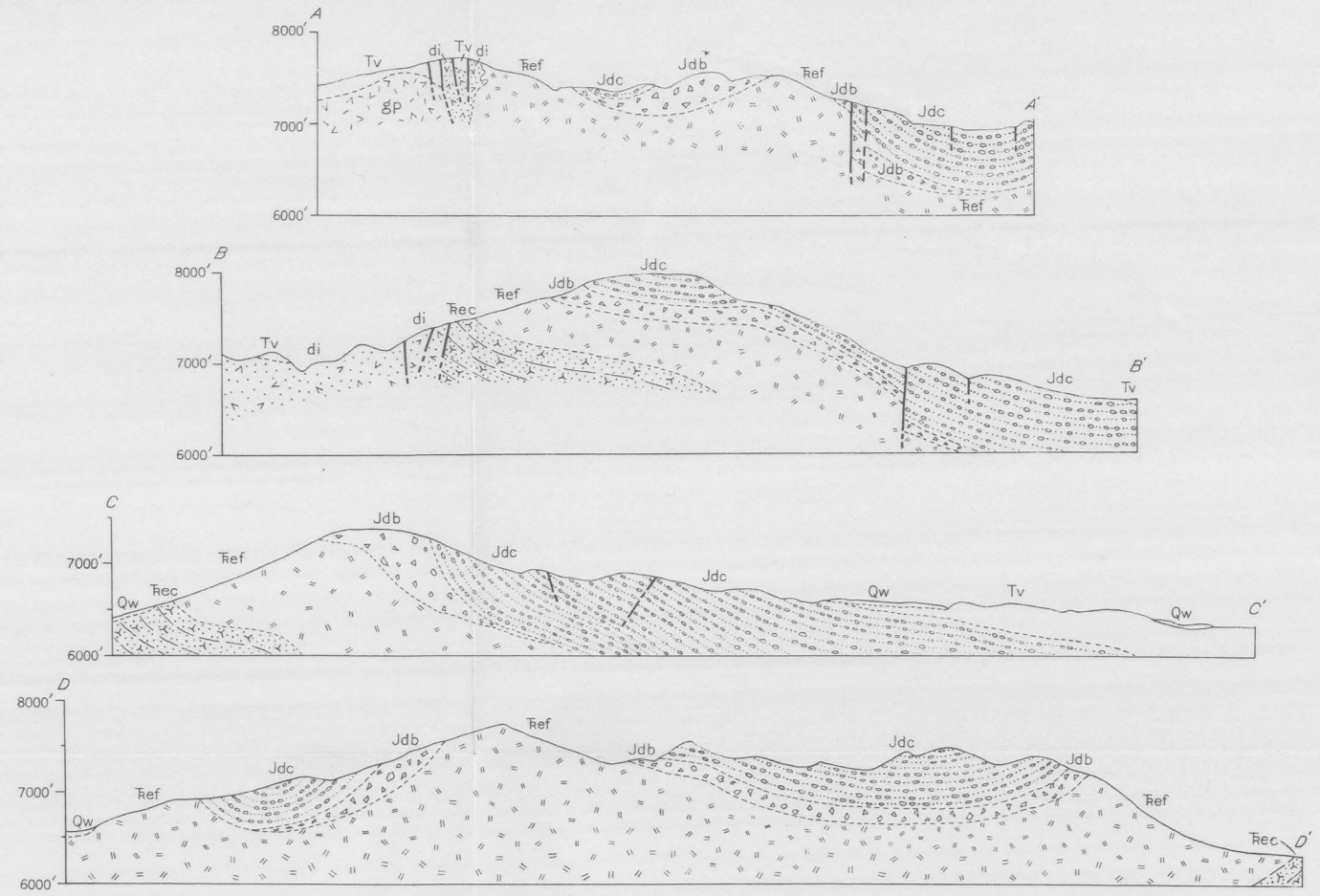
GEOLOGIC MAP AND SECTIONS OF PART OF THE GOLD RANGE DISTRICT, EXCELSIOR MOUNTAINS, NEVADA
