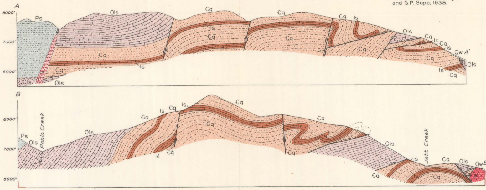
GEOLOGIC MAP AND SECTIONS BETWEEN JETT AND PABLO CANYONS, TOYABE RANGE, NEVADA
