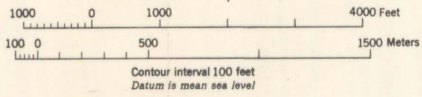
GEOLOGIC MAP AND SECTIONS BETWEEN JETT AND PABLO CANYONS, TOYABE RANGE, NEVADA
