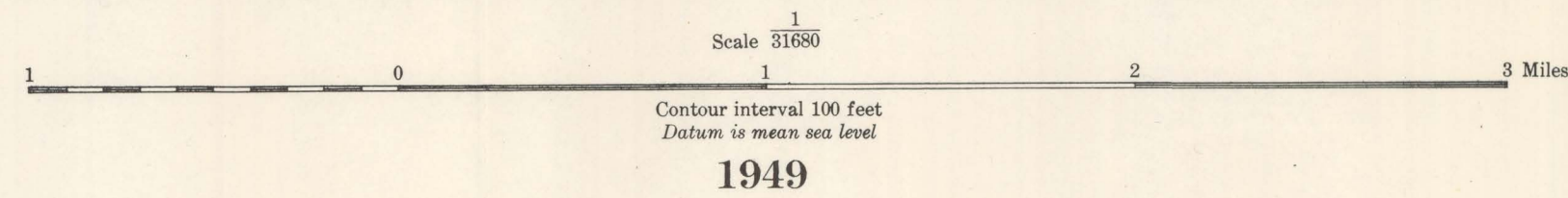
GEOLOGIC MAP AND STRUCTURE SECTIONS OF THE LA PLATA DISTRICT, COLORADO
