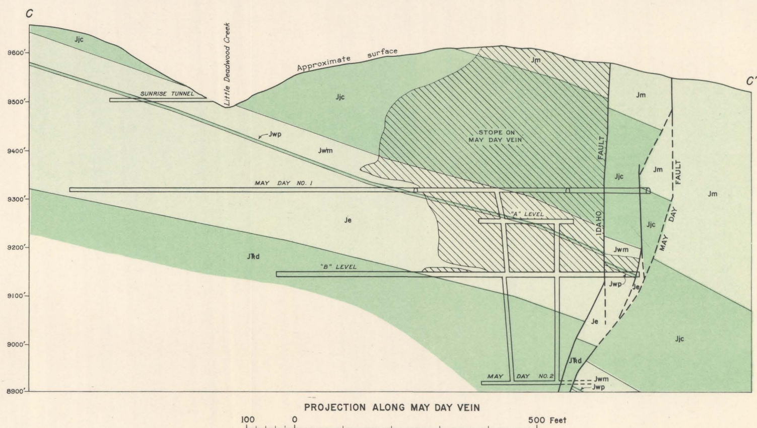
BLOCK DIAGRAM AND GENERALIZED SECTIONS, SHOWING GEOLOGY AND MINE WORKINGS OF MAY DAY AND IDAHO MINES
