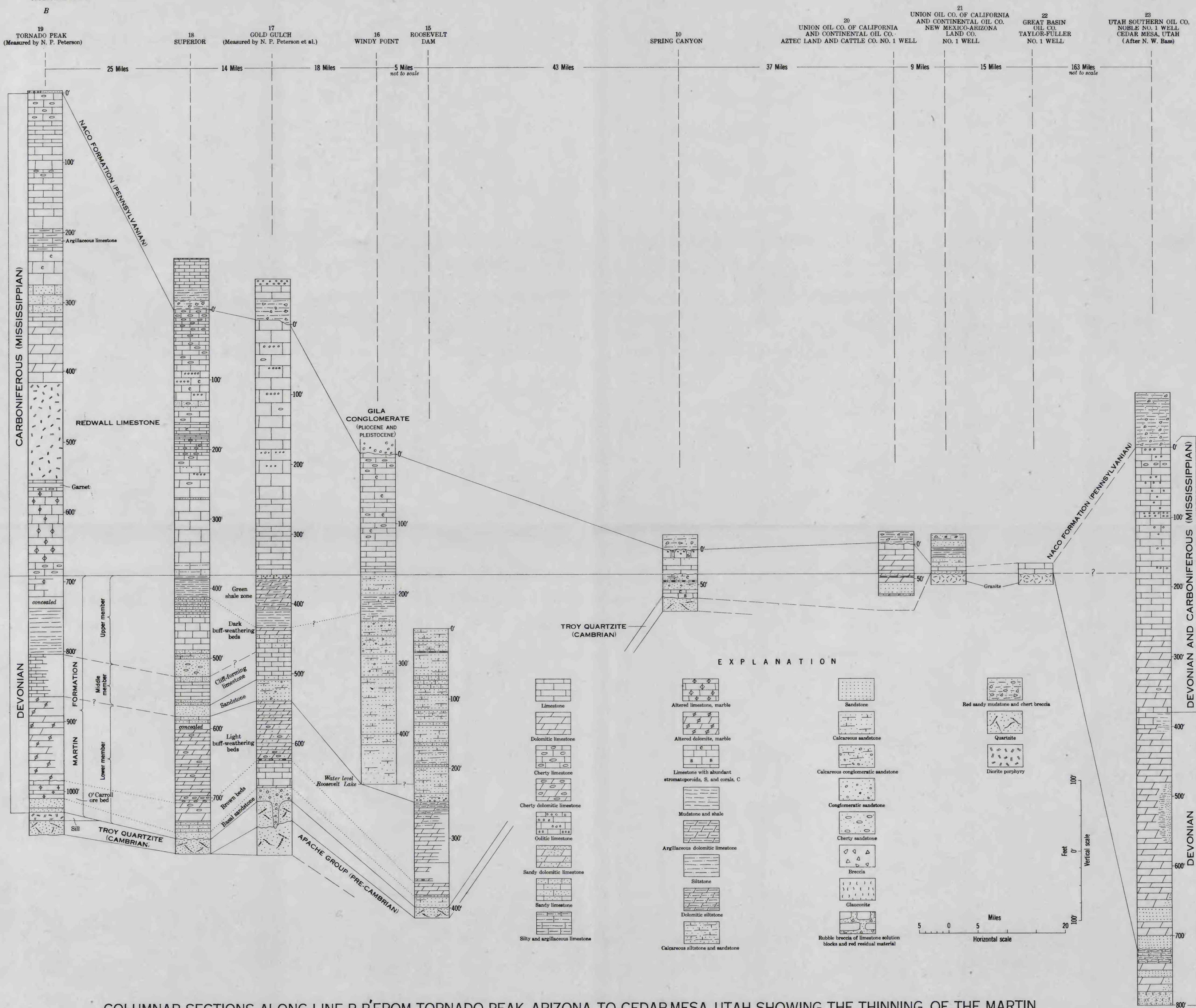
COLUMNAR SECTIONS ALONG LINE B-B' FROM TORNADO PEAK, ARIZONA, TO CEDAR MESA, UTAH SHOWING THE THINNING OF THE MARTIN FORMATION AND REDWALL LIMESTONE IN CENTRAL ARIZONA
