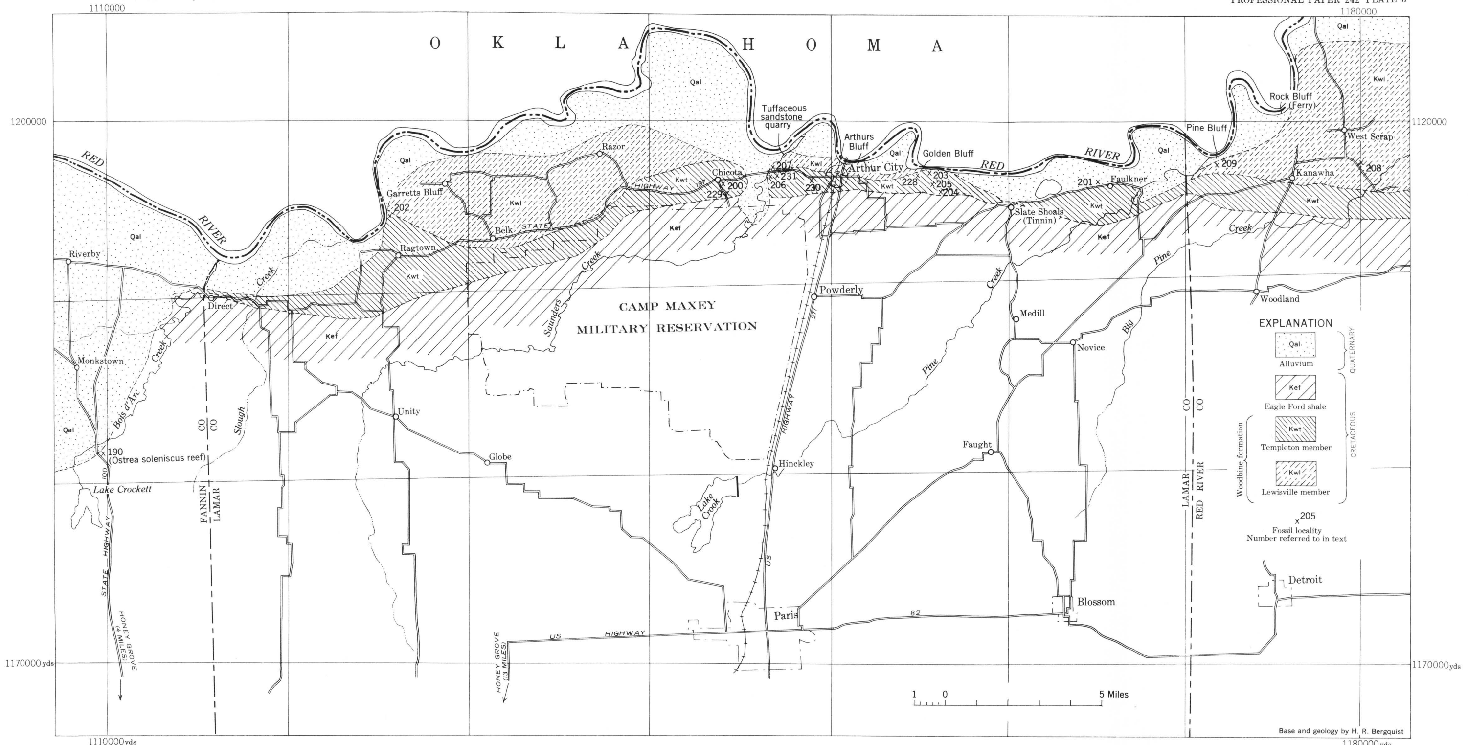
GEOLOGIC MAP OF PARTS OF FANNIN, LAMAR, AND RED RIVER COUNTIES, TEXAS, SHOWING FOSSIL-COLLECTING LOCALITIES
