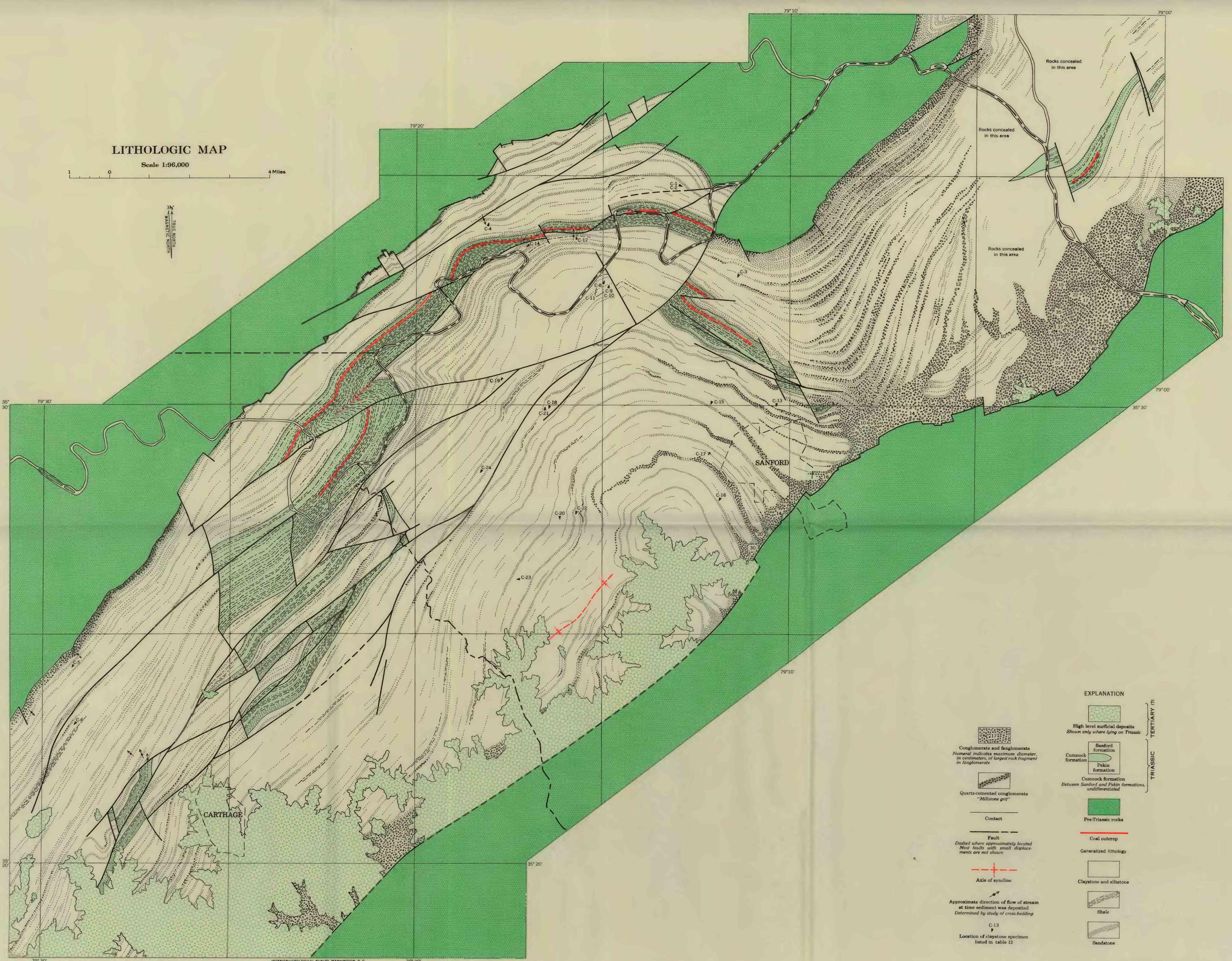
STRUCTURE AND LITHOLOGIC MAPS OF THE DEEP RIVER COAL FIELD, CHATHAM, LEE, AND MOORE COUNTIES, NORTH CAROLINA
