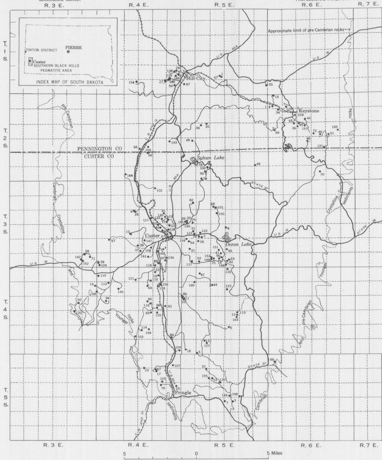
INDEX MAP SHOWING LOCATION OF PEGMATITE MINES AND PROSPECTS, SOUTHERN BLACK HILLS, SOUTH DAKOTA
