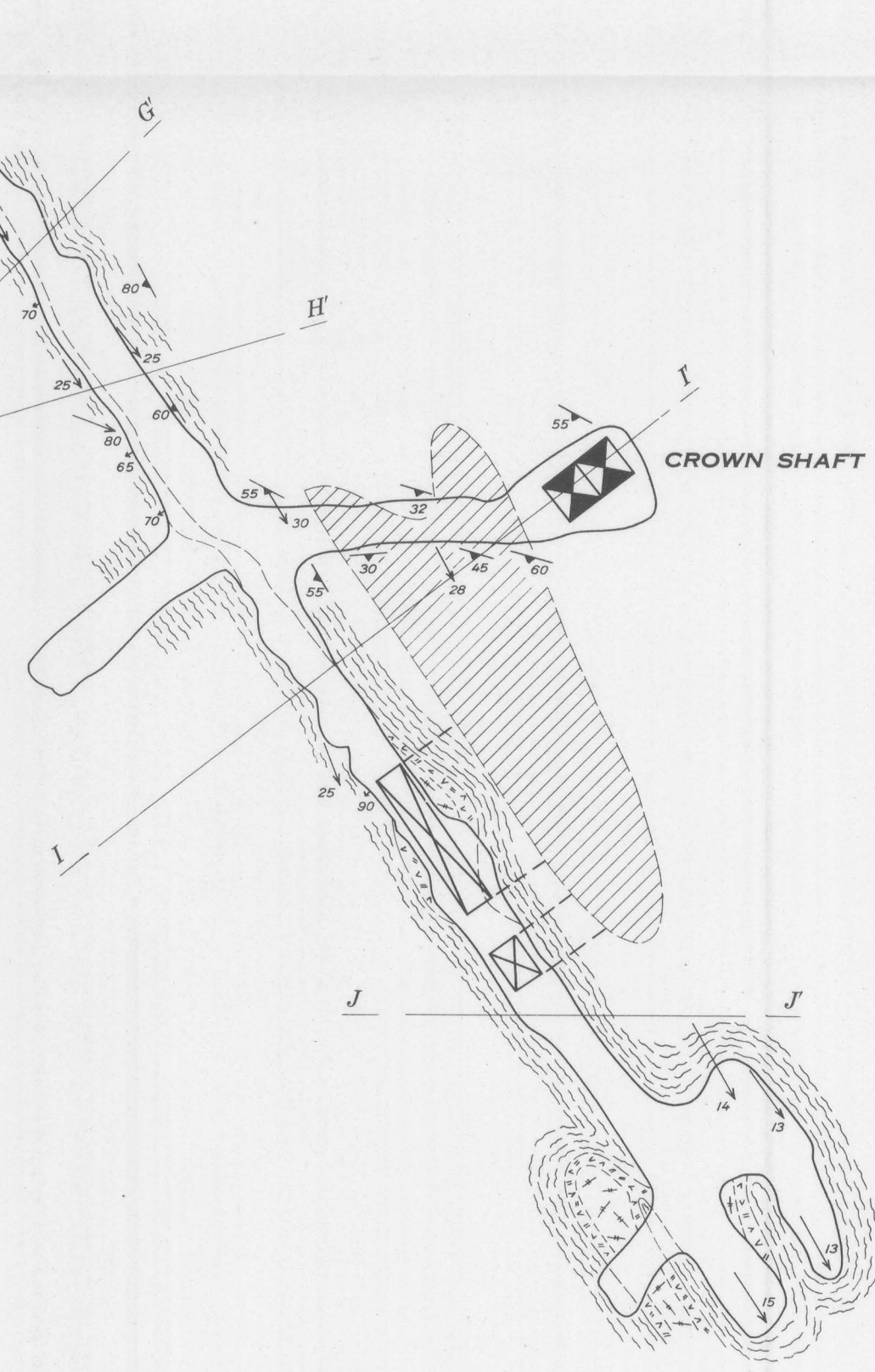
PLAN OF CROWN MINE 5686 LEVEL
