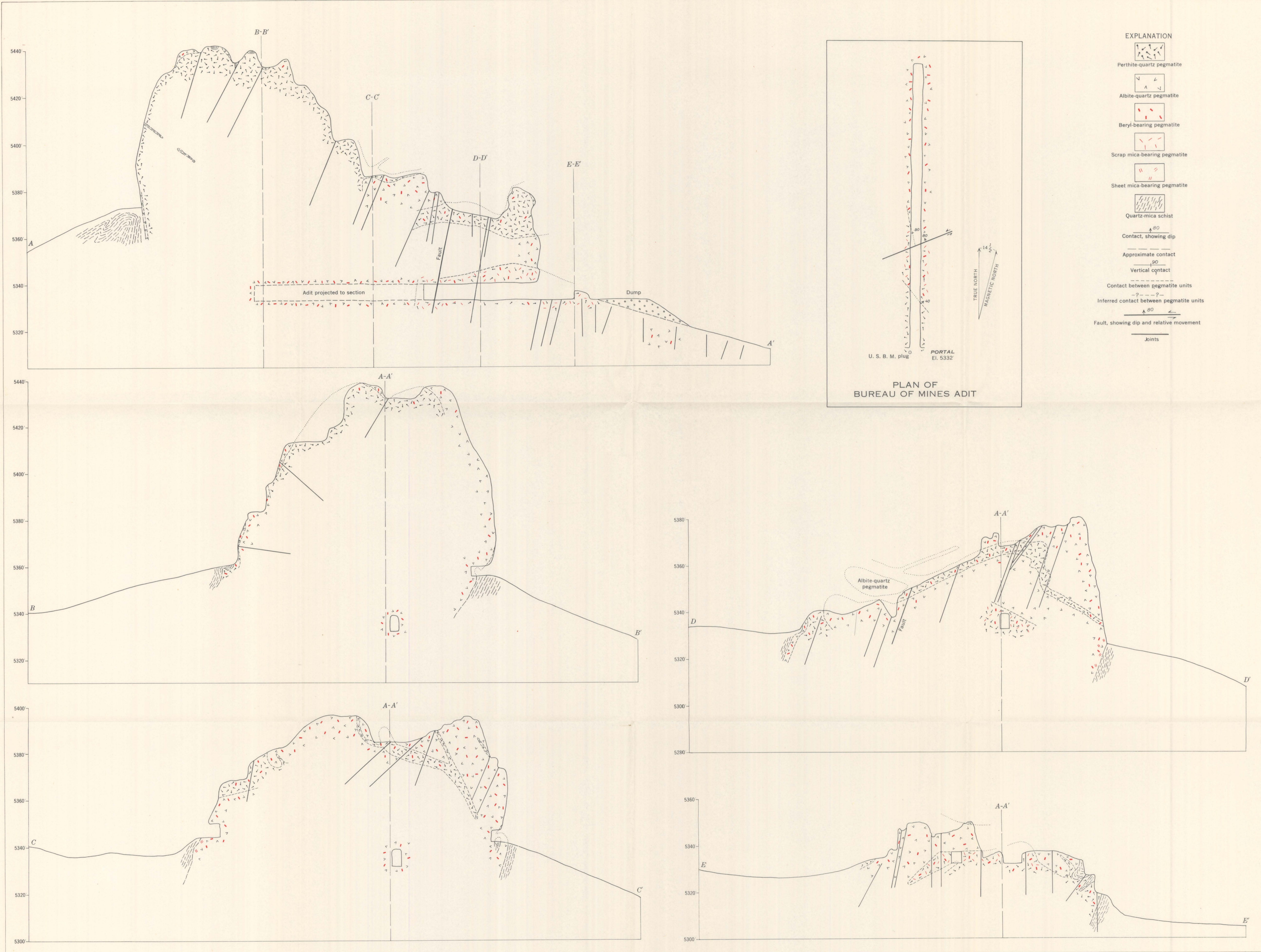
GEOLOGIC SECTIONS AND UNDERGROUND MAP, HELEN BERYL CLAIM, CUSTER COUNTY, SOUTH DAKOTA
