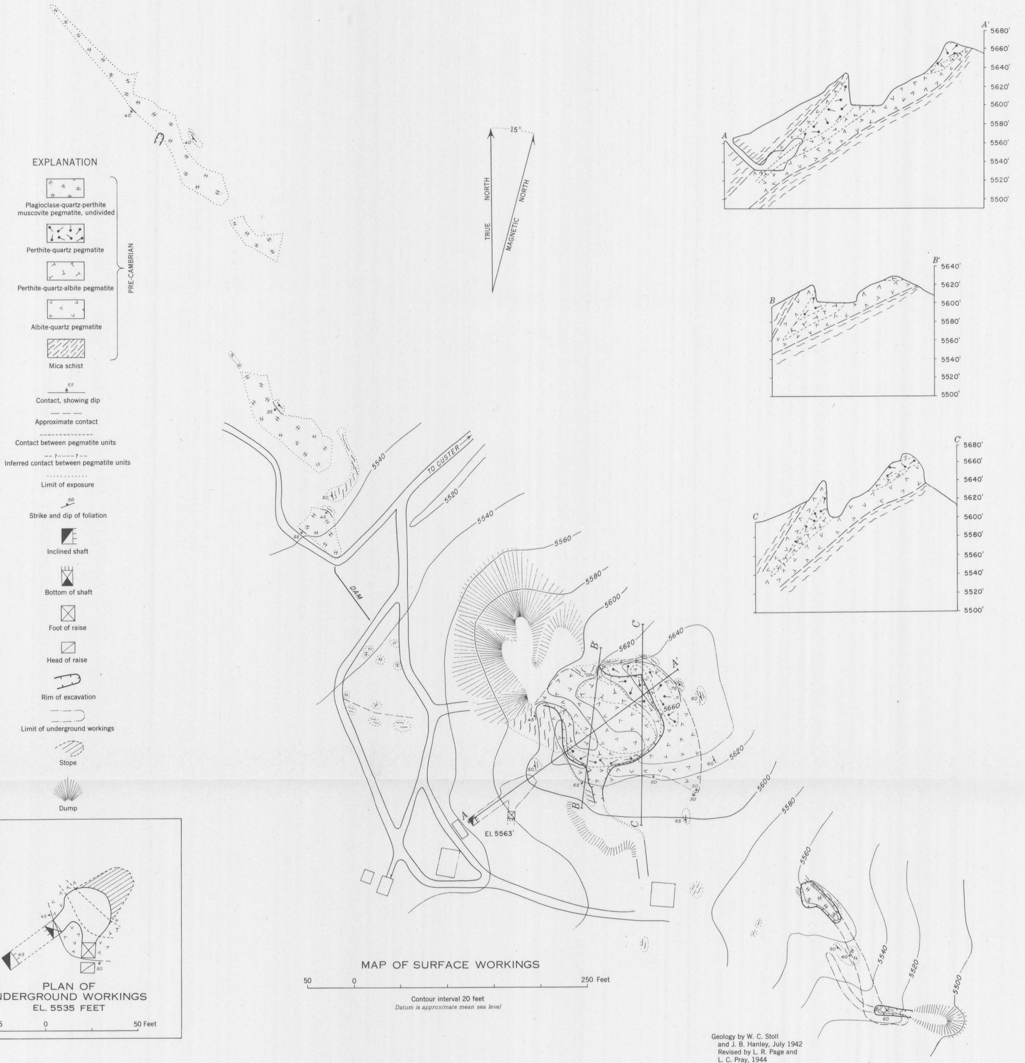
GEOLOGIC MAP AND SECTIONS, HIGHLAND LODGE (JOHN ROSS MINE), CUSTER COUNTY, SOUTH DAKOTA
