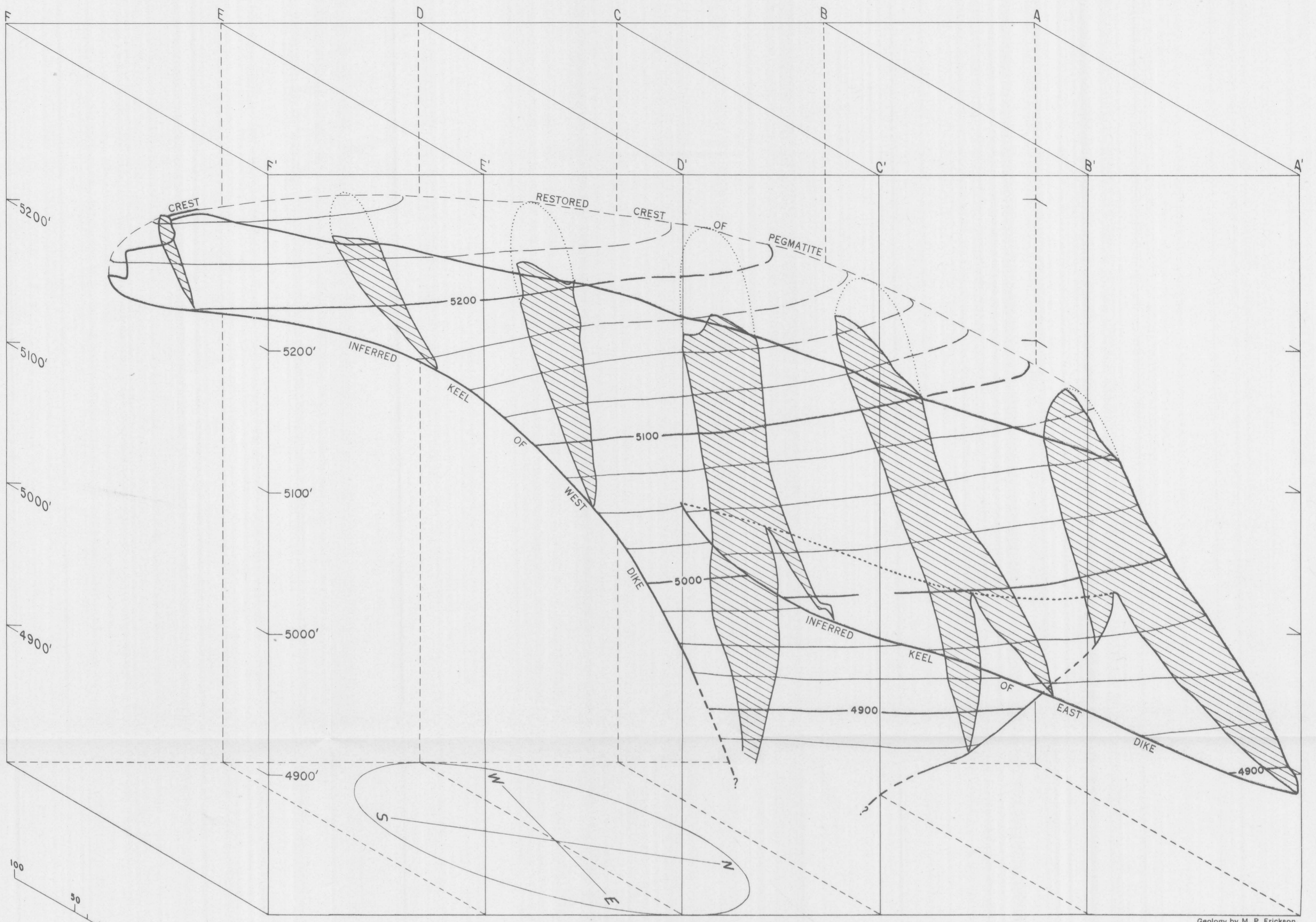
OBLIQUE PROJECTION
