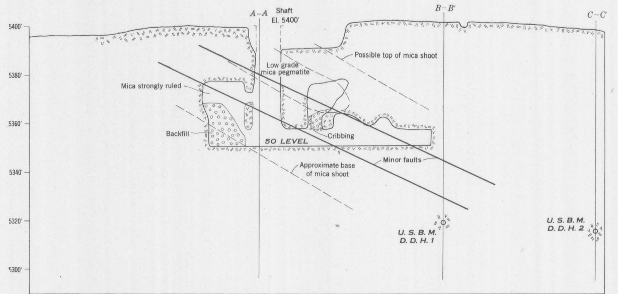
NORTH-SOUTH LONGITUDINAL SECTION INCLINED 75° TO THE WEST
