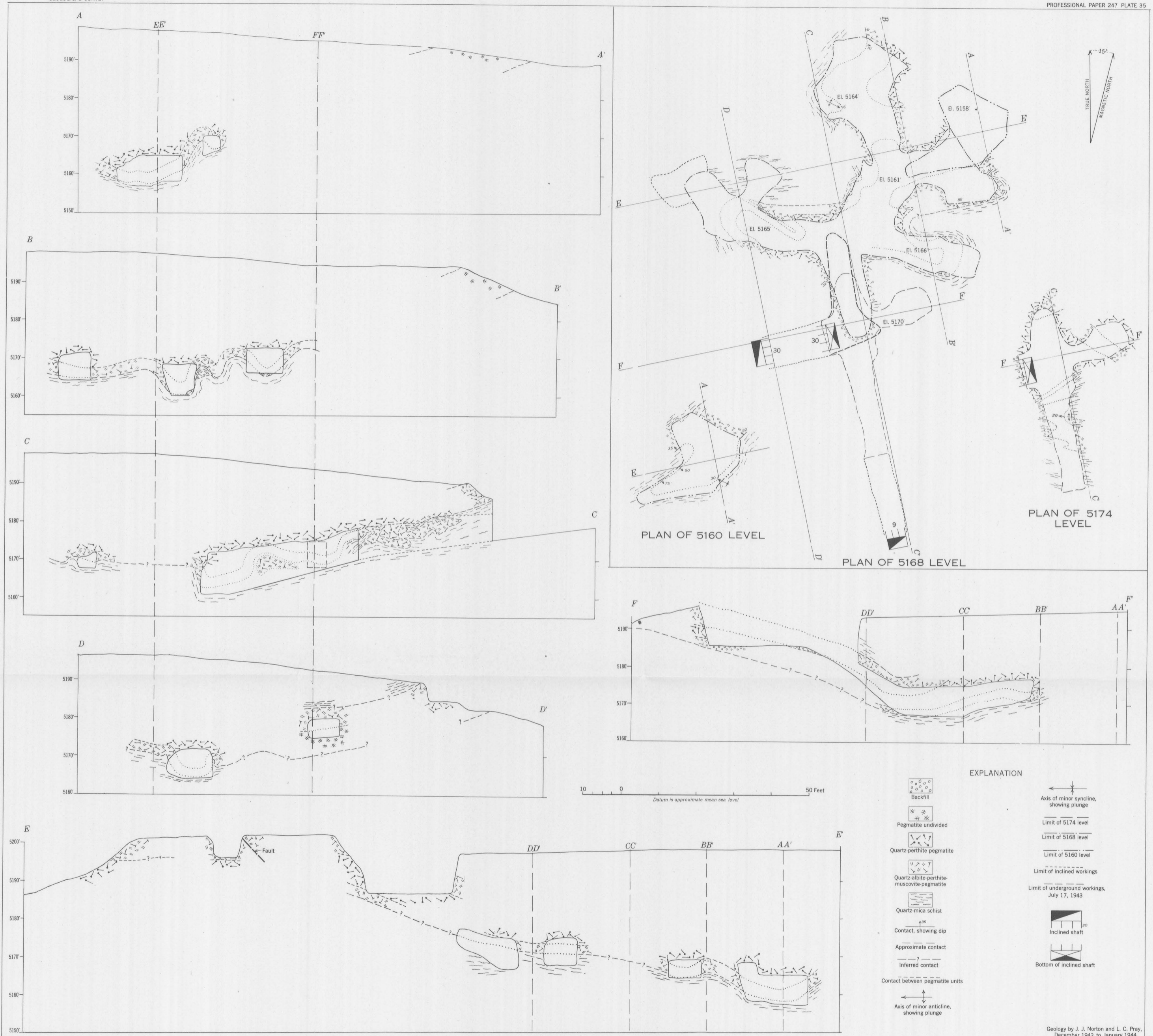
GEOLOGIC PLANS AND SECTIONS, AND UNDERGROUND WORKINGS, RED DEER MICA MINE, CUSTER COUNTY, SOUTH DAKOTA
