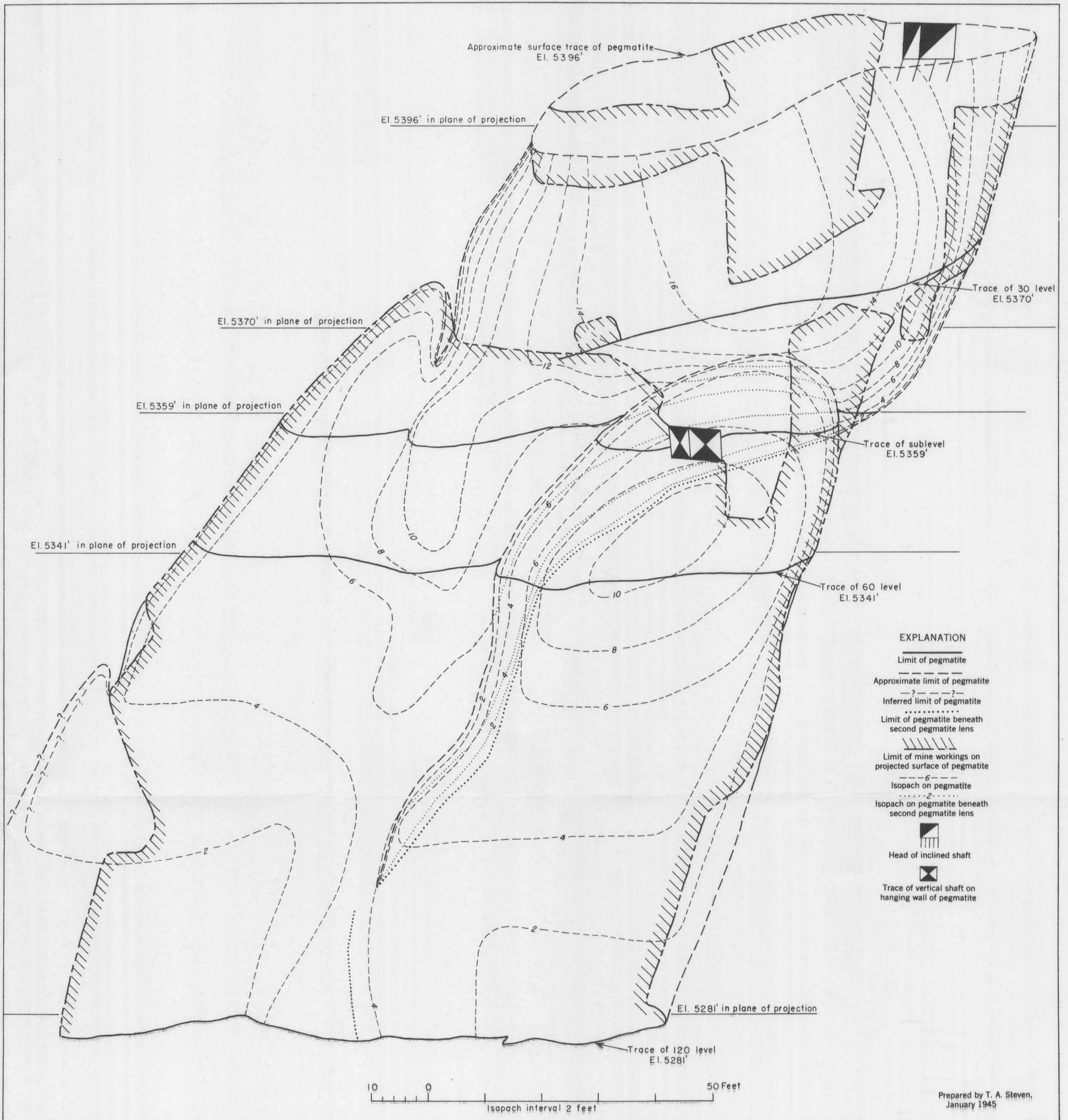
ISOPACH MAP OF THE VICTORY MICA MINE, CUSTER COUNTY, SOUTH DAKOTA
