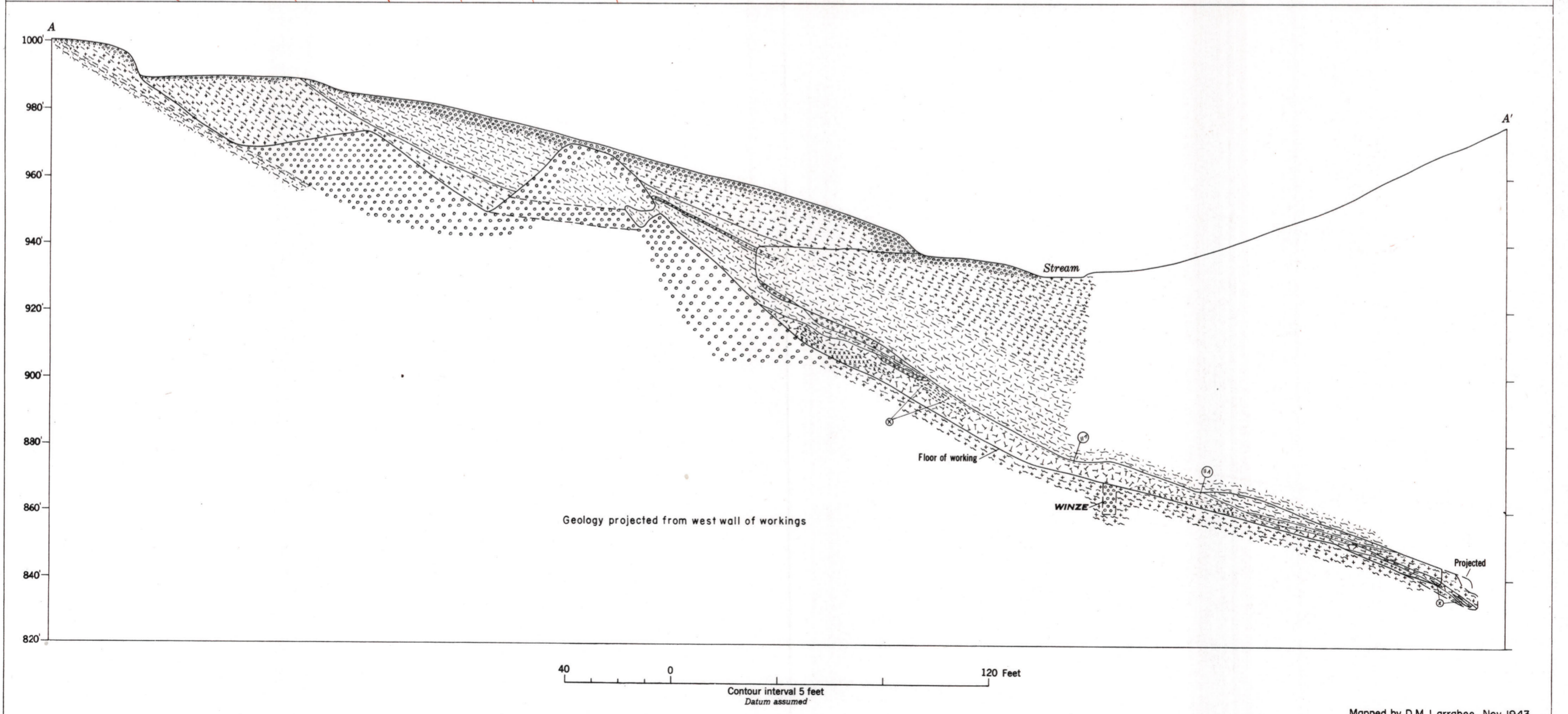
GEOLOGIC MAP AND SECTIONS OF THE HAWKINS MINE, STOKES COUNTY, NORTH CAROLINA
