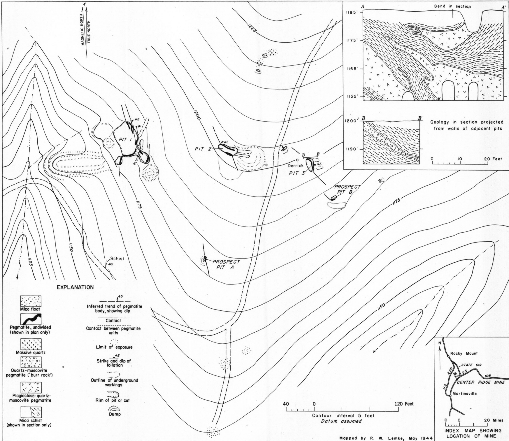
GEOLOGIC MAP AND SECTIONS OF THE CENTER RIDGE MINE, FRANKLIN COUNTY, VIRGINIA
