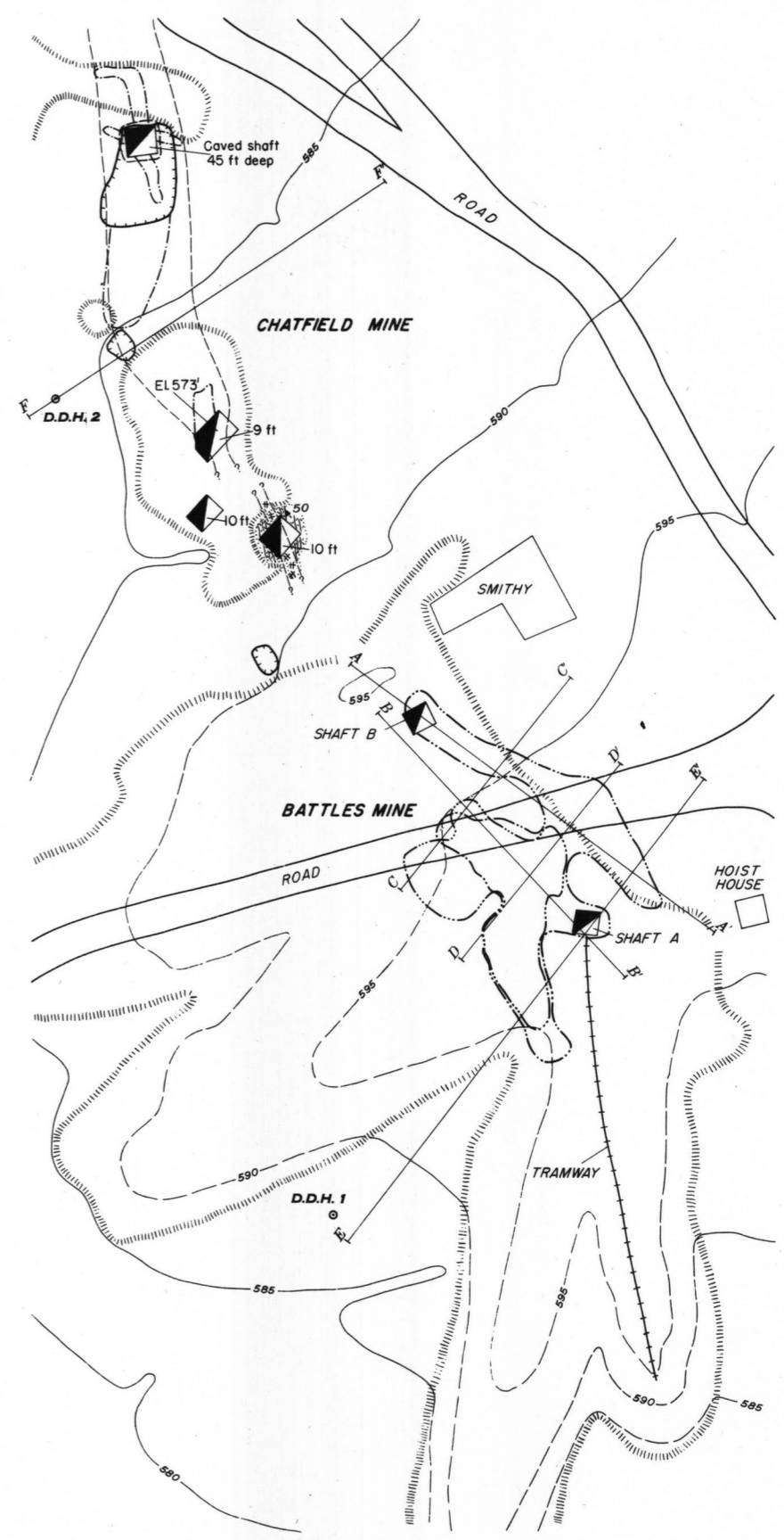
GEOLOGIC MAP, PLANS, AND SECTIONS OF THE BATTLES AND CHATFIELD MINES, MONROE COUNTY, GEORGIA
