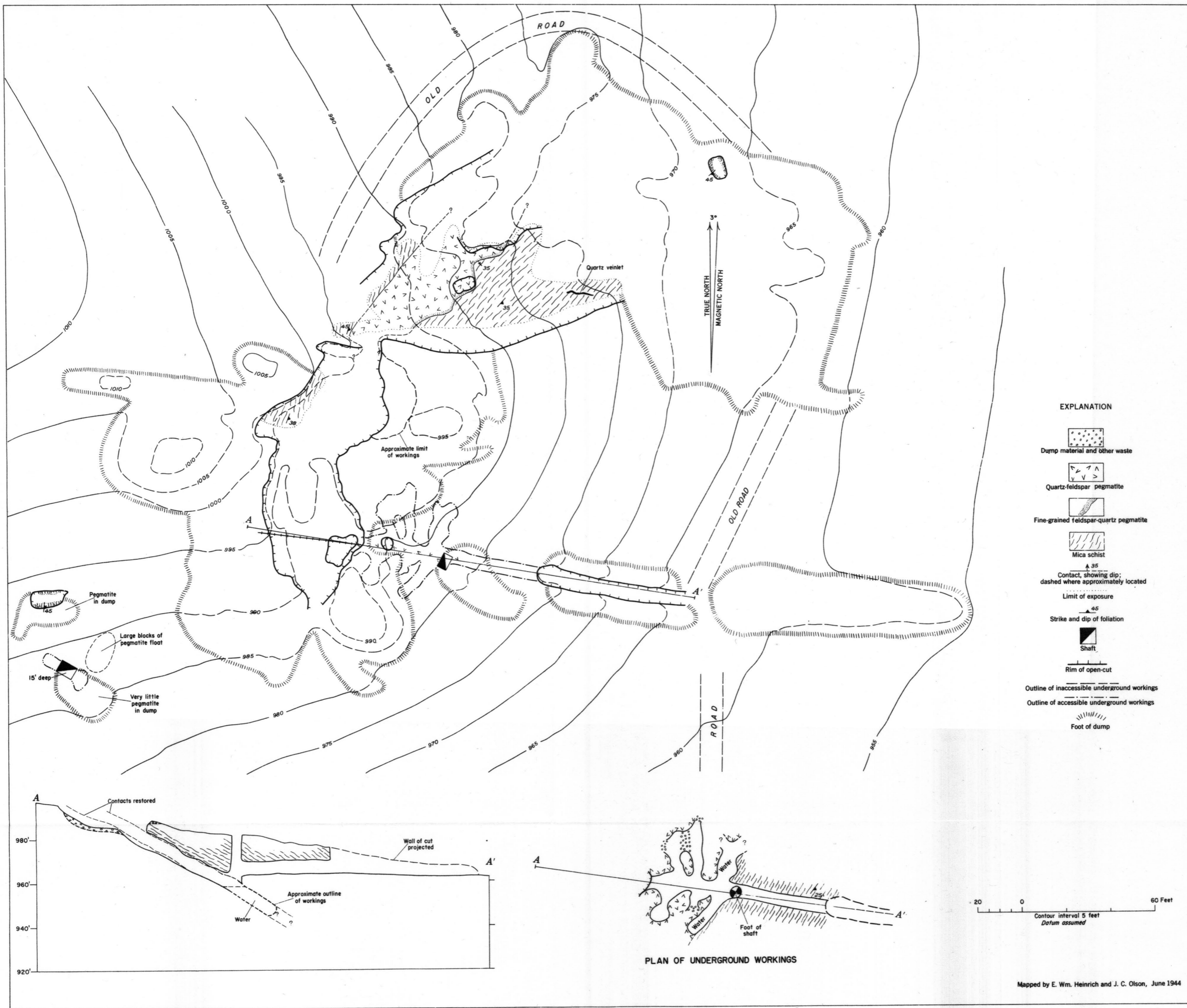
GEOLOGIC MAP, PLAN, AND SECTION OF THE ARNOTT MINE, RANDOLPH COUNTY, ALABAMA
